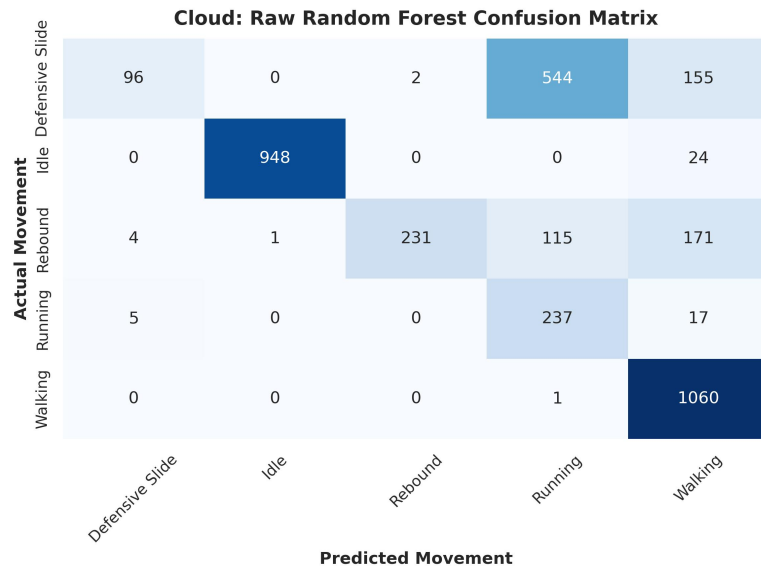
Figure 5.12: Confusion Matrix for the Random Forest Model before Smoothing
