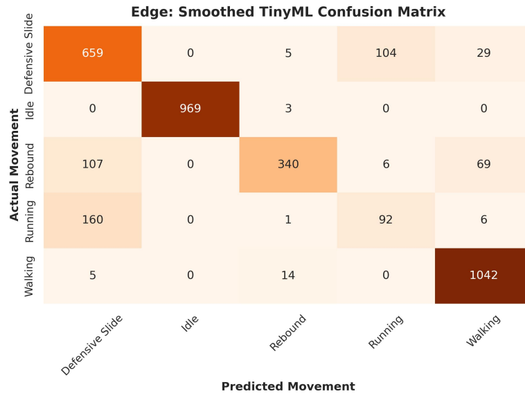
Figure 5.15: Confusion Matrix for the Smoothed TinyML Model
