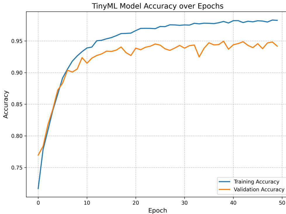
Figure 5.3: TinyMLAccuracy
