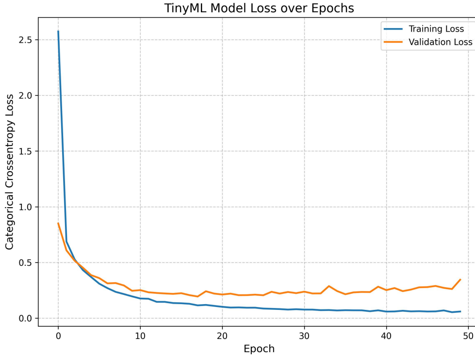
Figure 5.4: TinyMLLoss
