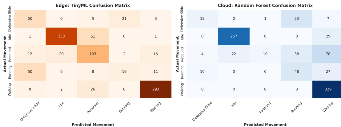
Figure 5.10: Confusion Matrices for TinyML (Left) and Random Forest (Right)
