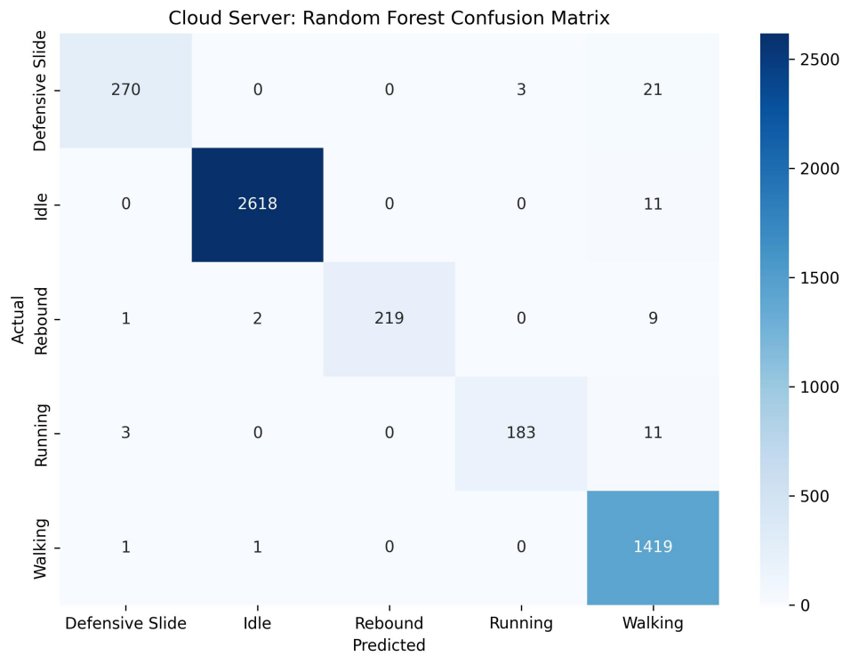
Figure 5.7: Random ForestL Confusion Matrix
