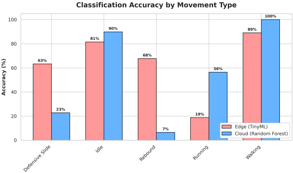
Figure 5.11: Classification Accuracy Segmented by Target Movement
