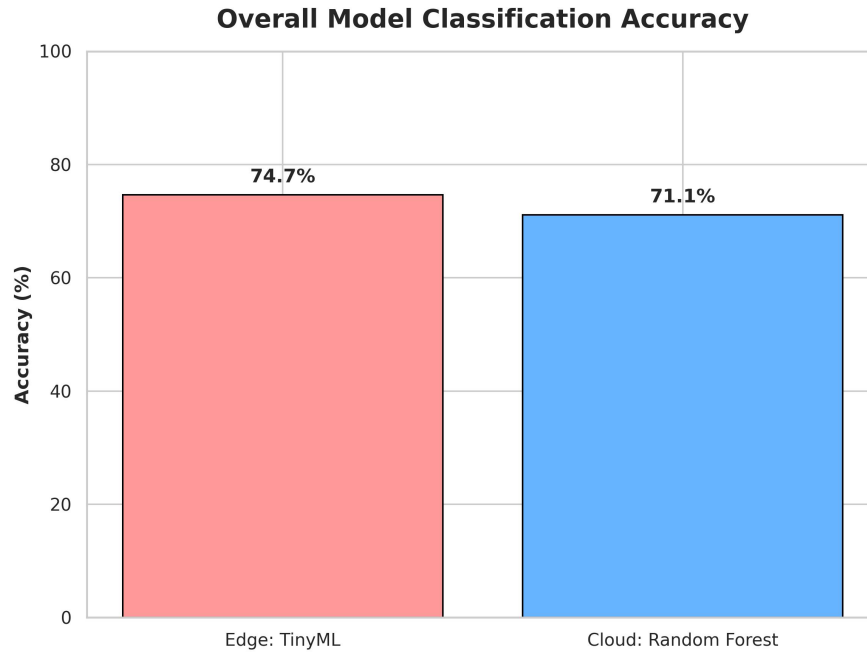
Figure 5.9: Overall Classification Accuracy: Local TinyML vs. Cloud Random Forest
