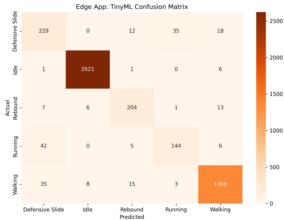
Figure 5.6: TinyML Confusion Matrix
