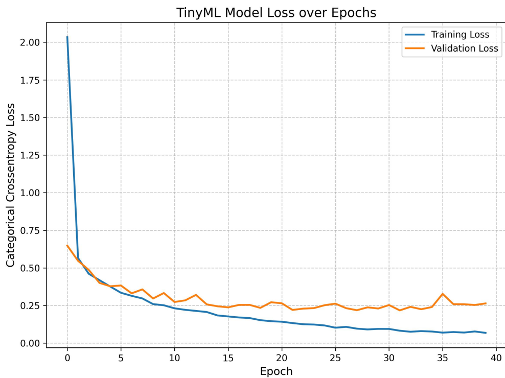
Figure 5.4: TinyMLLoss
