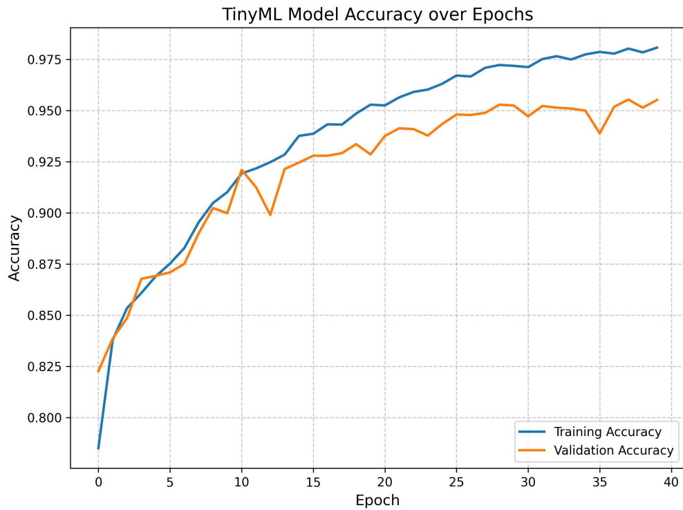
Figure 5.3: TinyMLAccuracy
