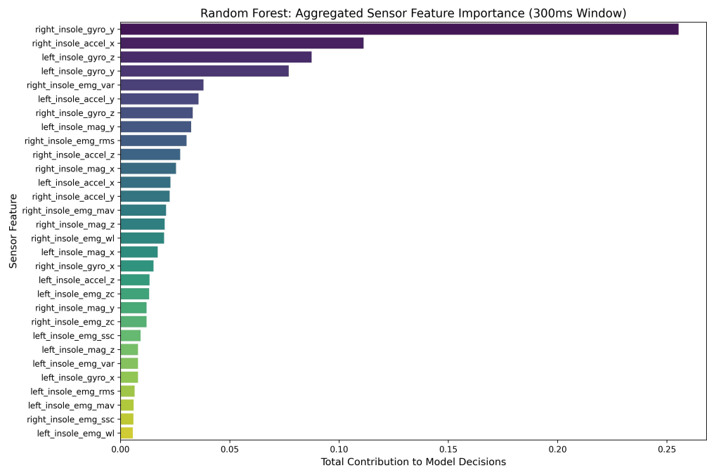
Figure 5.5: Feature Importance Graph
