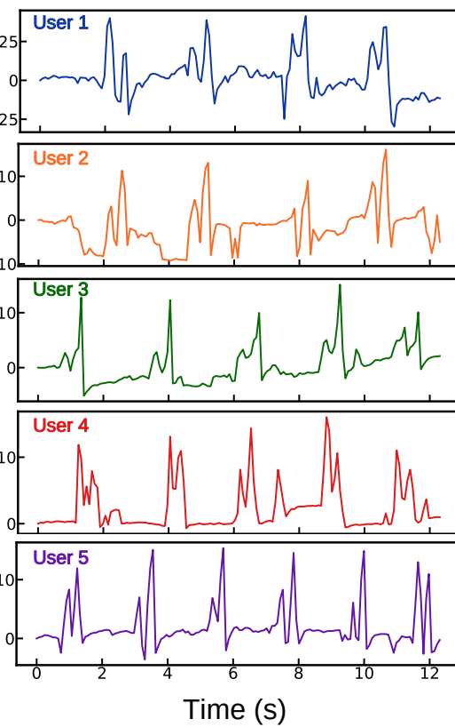
Raw pressure-time signals across users
