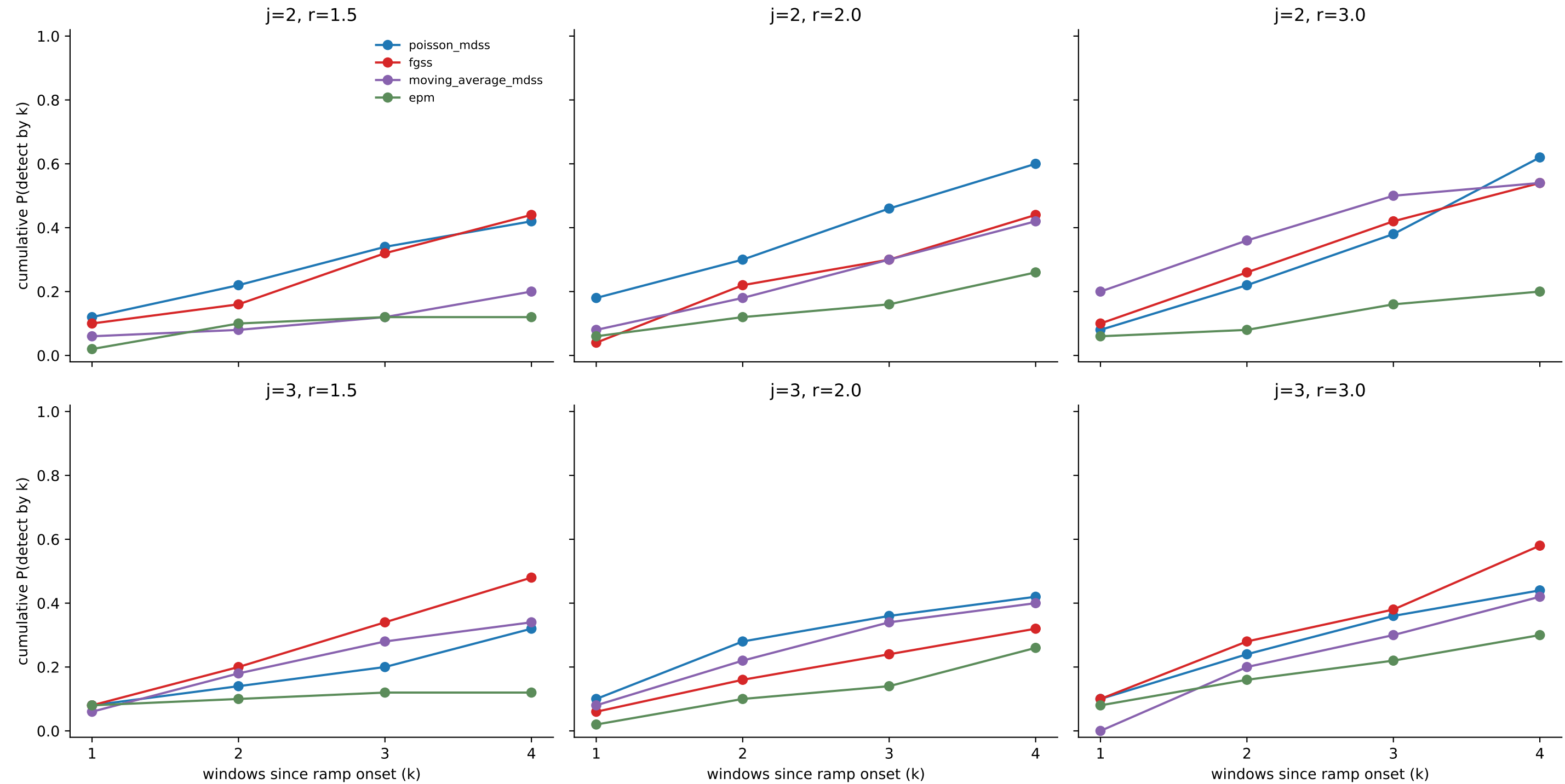
Censoring-safe detection curves: cumulative P(detect) vs windows-since-onset (M=999, RAMP_TRIALS=50)
