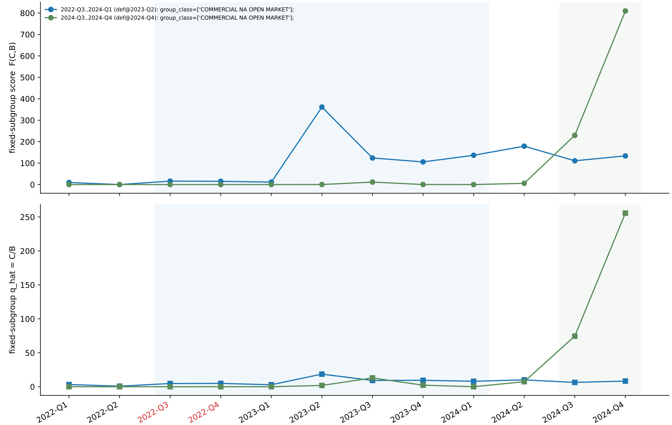
E3 persistent-family emergence: a FIXED subgroup's score & q_hat across the test period (shaded = family span; red x-labels = thin window)
