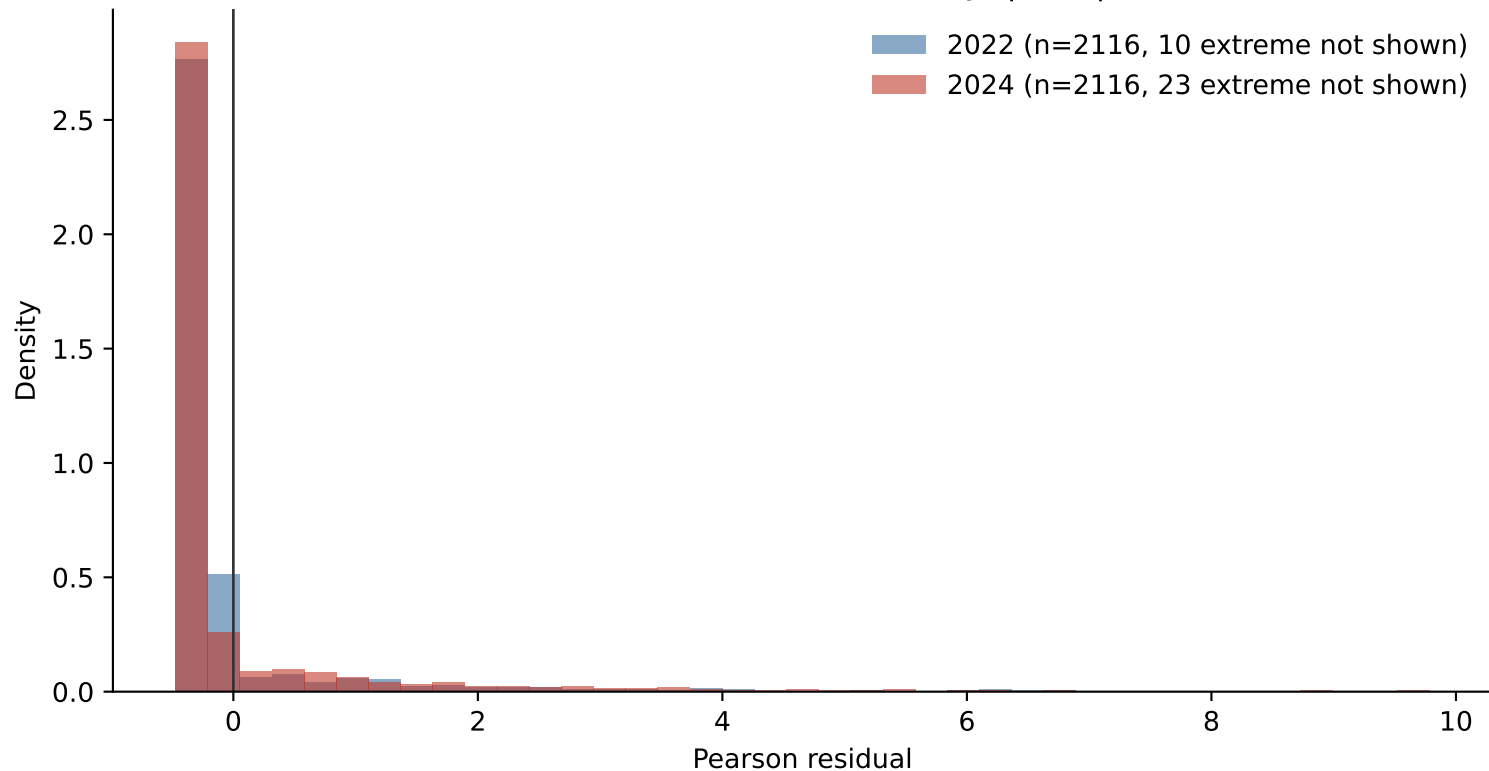
Per-cell Pearson residual, scoreable cells only ( |\text{resid}| \leq 10 shown)
