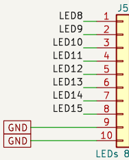
LEDs 8-15
