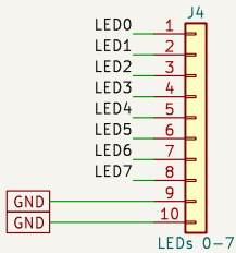
LEDs 0-7
