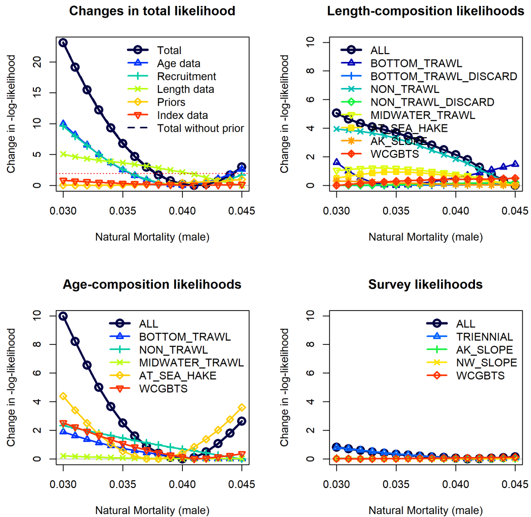
Figure 170: Male natural mortality ( M ) likelihood profile for each of the likelihood components.
