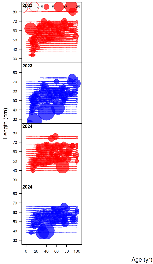
Figure 96: Pearson residuals of conditional age at length fits for the at-sea-hake fishery in the years 2023-2024. Closed bubble are positive residuals (observed > expected) and open bubbles are negative residuals (observed < expected).
