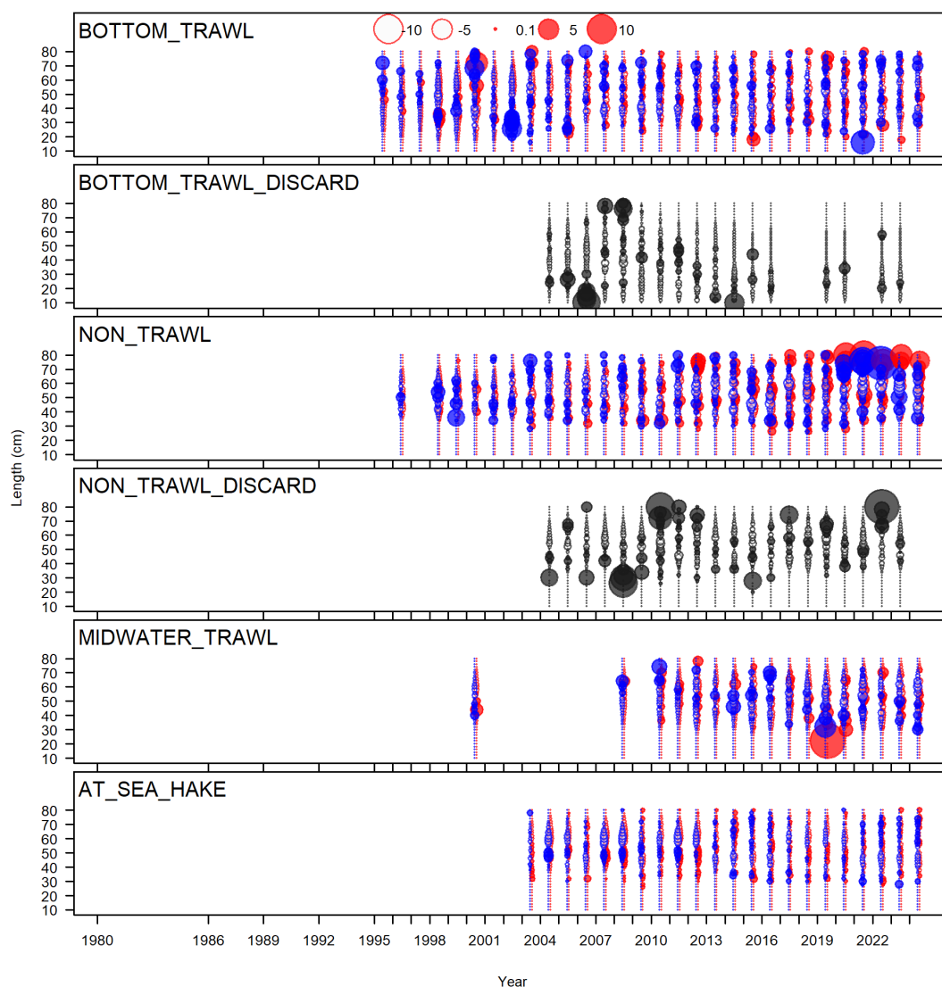
Figure 79: Pearson residuals of length fits for each fishing fleet. Closed bubble are positive residuals (observed > expected) and open bubbles are negative residuals (observed < expected).
