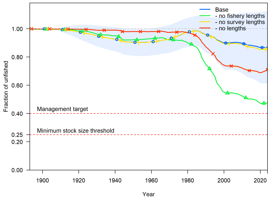
Figure 150: Relative spawning output (fraction unfished) across data removal sensitivities (length compositions by source).
