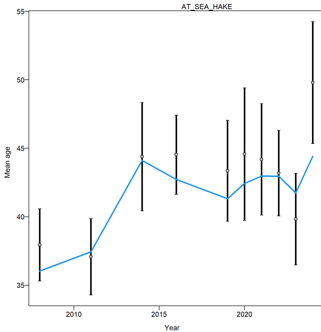
Figure 103: Mean age from conditional age-at-length data for the at-sea-hake fishery with 95% confidence intervals based on current samples sizes and data weighting.
