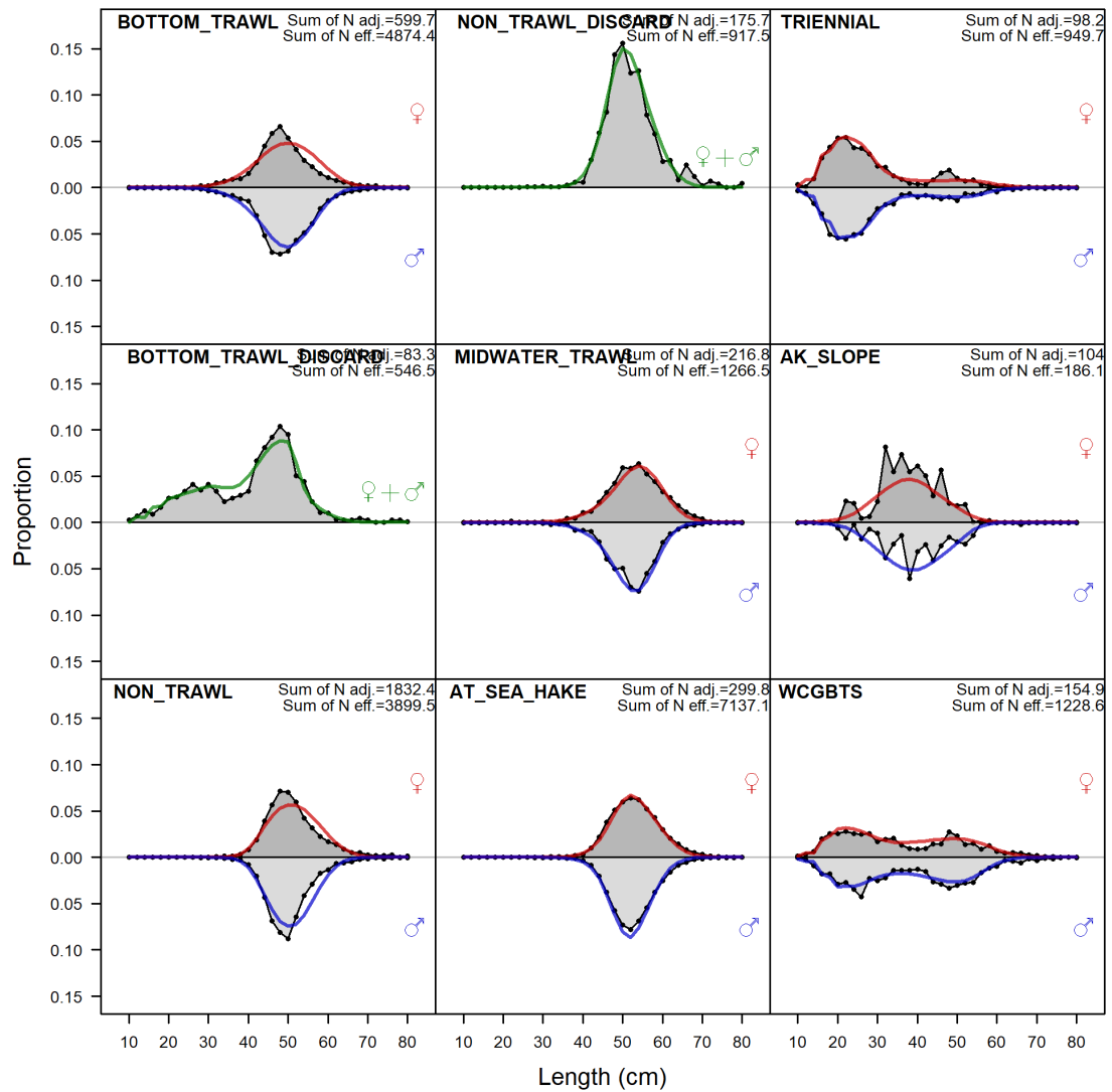
Figure 163: Aggregate fit to length compositions for the scenario that assume logistic selectivity for all fisheries and time blocks.
