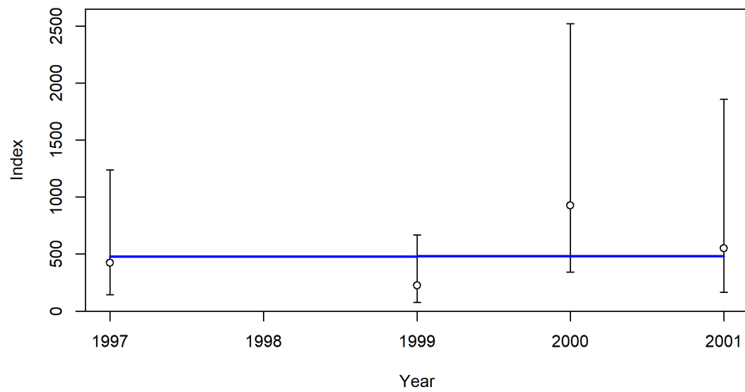
Figure 128: Fit to index data for the Alaska Slope survey. Lines indicate 95% uncertainty interval around index values based on the assumption of lognormal error.
