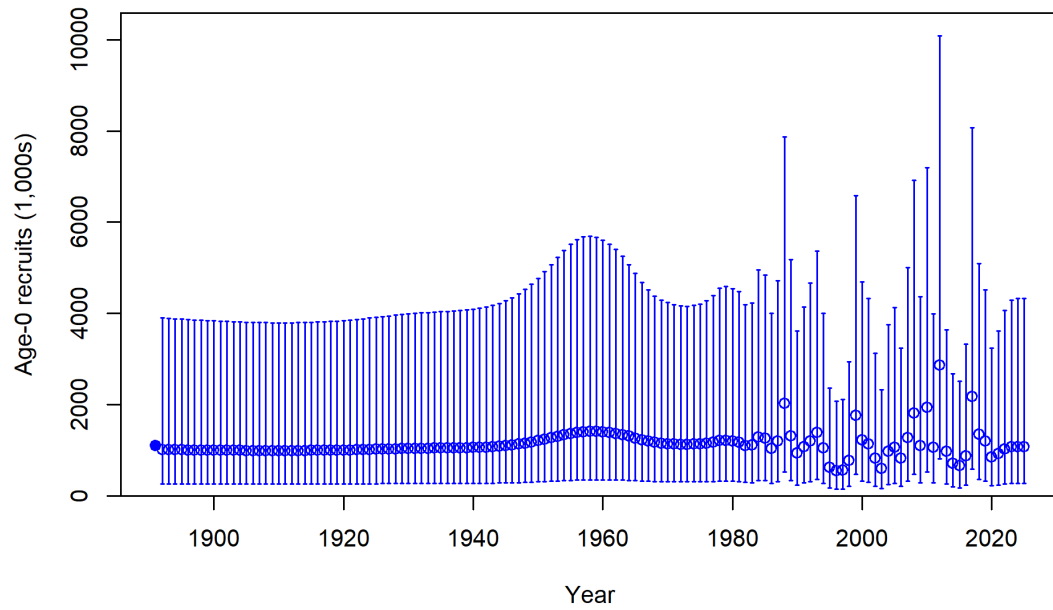
Figure 141: Estimated time series of age-0 recruits for the base model.
