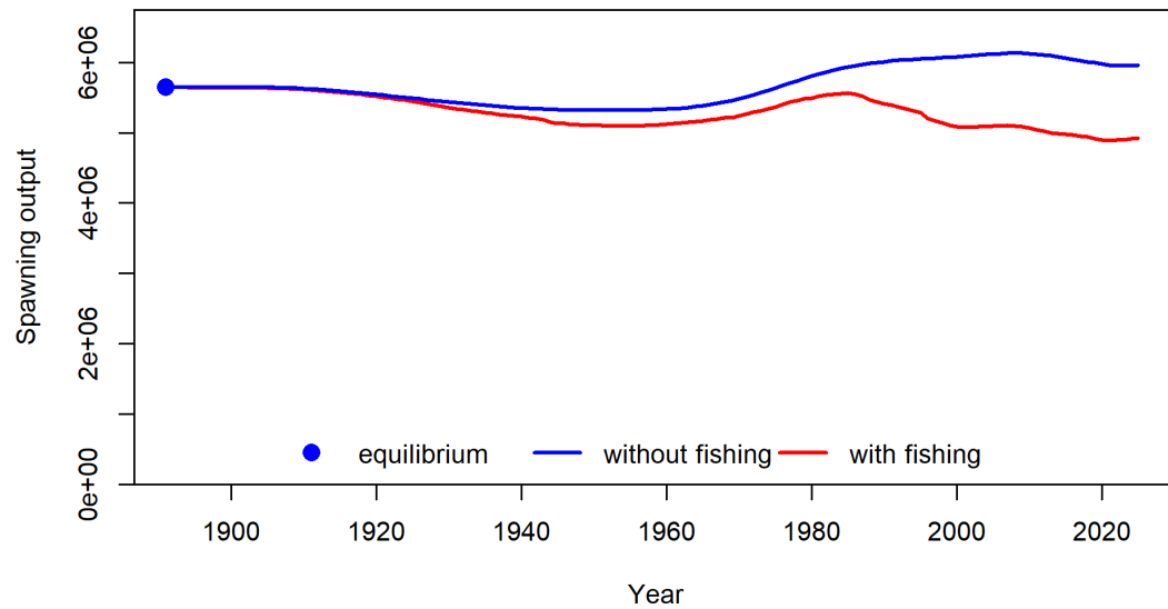
Figure 178: Dynamic B0 plot. The lower line shows the time series of estimated spawning output in the presence of fishing mortality. The upper line shows the time series that could occur under the same dynamics (including deviations in recruitment), but without fishing. The point at the left represents the unfished equilibrium.
