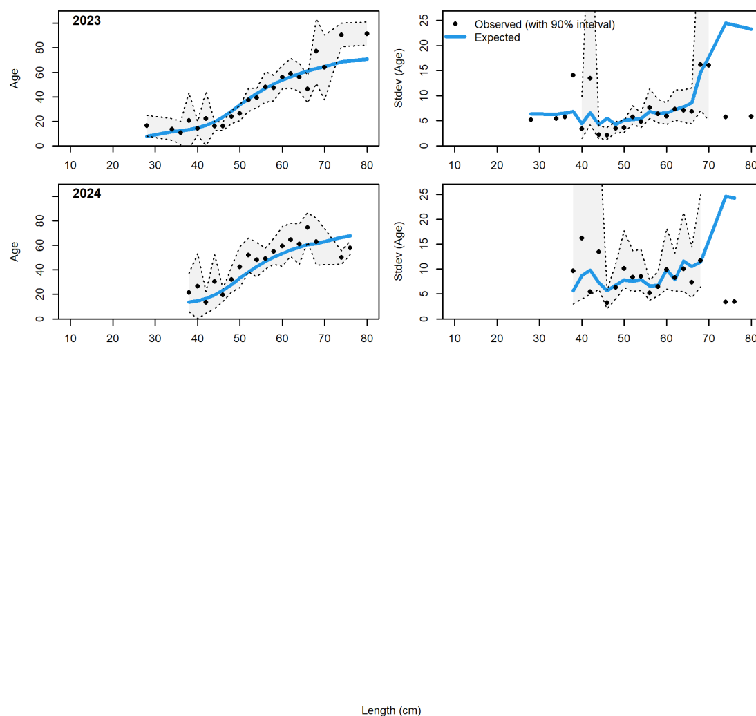
Figure 115: Conditional age at length plot showing mean age (left panels) and standard deviation (right panels) for the at-sea-hake fishery in years 2023-2024. The CIs are 90% based on adding 1.64 SE of mean to the data for the left panels and the standard error of mean age at length (obs. and exp.) with 90% CIs based on the chi-square distribution.
