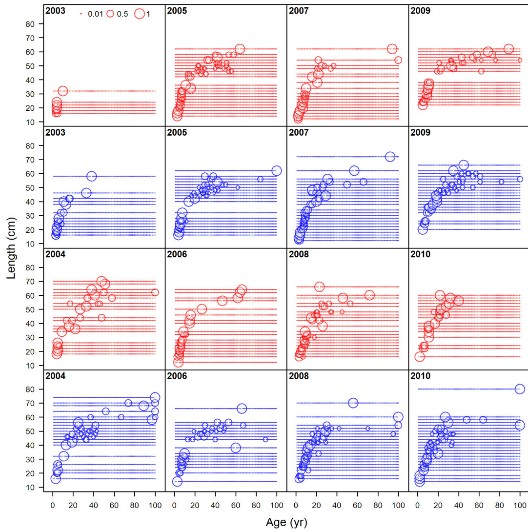
Figure 29: Conditional ages-at-length composition data for WCGBTS.
