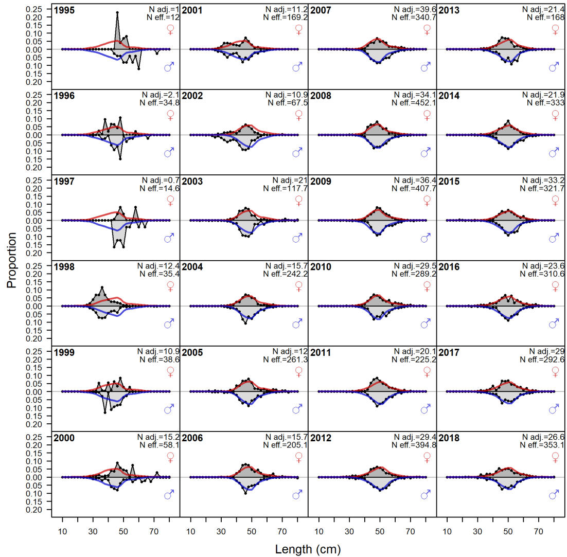
Figure 68: Observed (gray density plot) and expected (density lines by sex) length compositions by year for the bottom trawl fishery in years available between 1995-2018. 'N adj.' is the input sample size after data-weighting adjustment. N eff. is the calculated effective sample size used in the McAllister-Ianelli tuning method.
