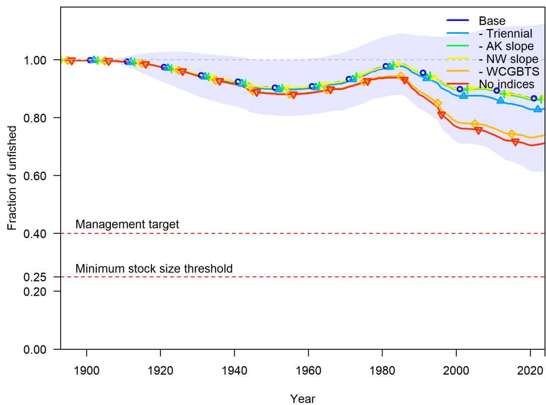
Figure 146: Relative spawning output (fraction unfished) across data removal sensitivities (indices).
