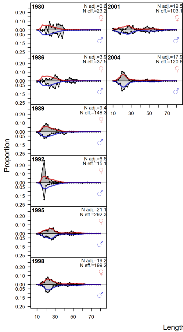
Figure 76: Observed (gray density plot) and expected (density lines by sex) length compositions by year for the Triennial Bottom Trawl Survey in years available between 1980-2004. 'N adj.' is the input sample size after data-weighting adjustment. N eff. is the calculated effective sample size used in the McAllister-Ianelli tuning method.
