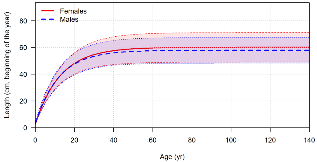
Figure 131: Estimated age and growth relationship in the reference model .Shaded area indicates 95% distribution of length at age around estimated growth curve.
