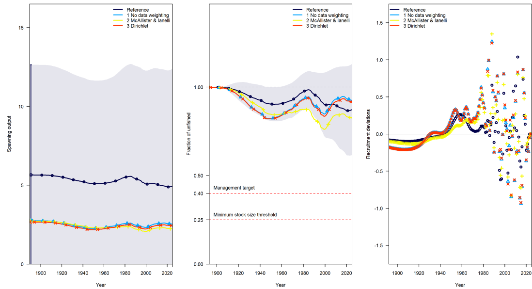
Figure 154: Comparison of spawning output (left panel), relative stock status (middle panel) and recruitment estimation (right panel) for models under different data weighting scenarios. The reference model uses the Francis method.
