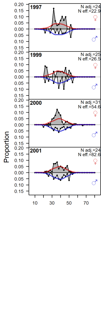
Figure 77: Observed (gray density plot) and expected (density lines by sex) length compositions by year for the Alaskan Slope Bottom Trawl Survey in years available between 1997-2001. 'N adj.' is the input sample size after data-weighting adjustment. N eff. is the calculated effective sample size used in the McAllister-Ianelli tuning method.
