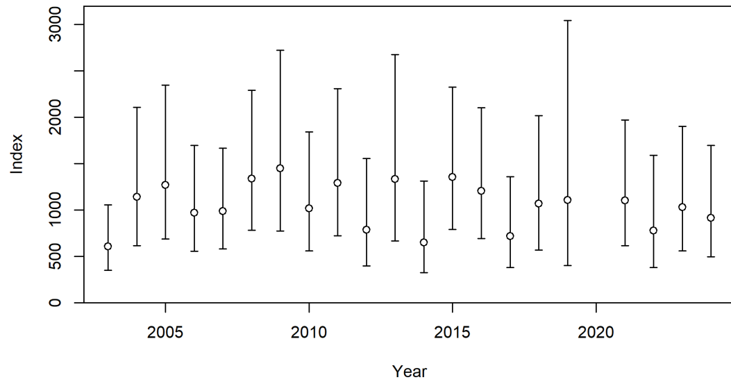
Figure 34: WCG BTS index.
