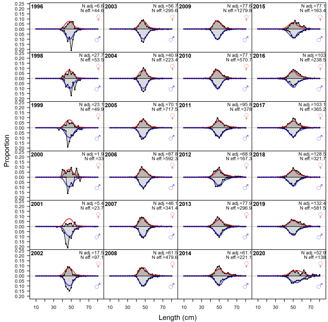
Figure 71: Observed (gray density plot) and expected (density lines by sex) length compositions by year for the non-trawl fishery in years available between 1996-2020. 'N adj.' is the input sample size after data-weighting adjustment. N eff. is the calculated effective sample size used in the McAllister-Ianelli tuning method.
