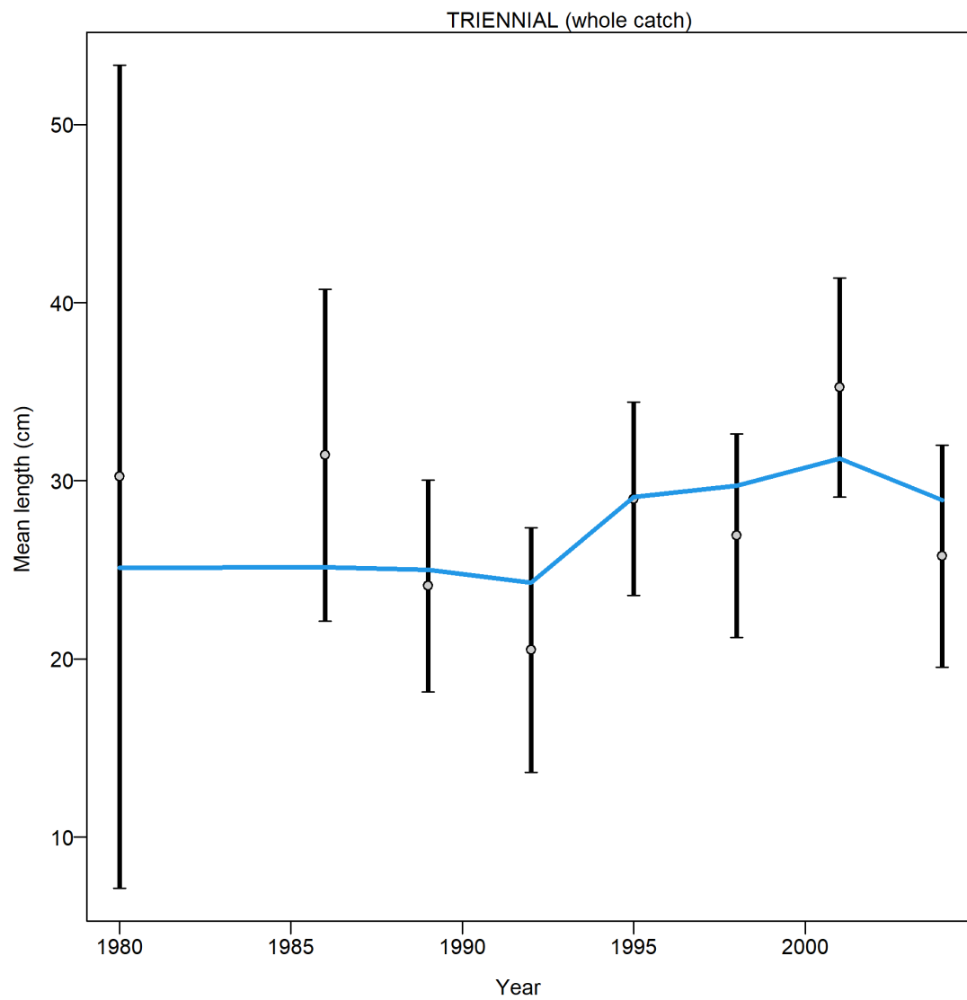
Figure 87: Mean length (cm) index from the Triennial survey with 95 percent confidence intervals based on sample sizes and data weighting.
