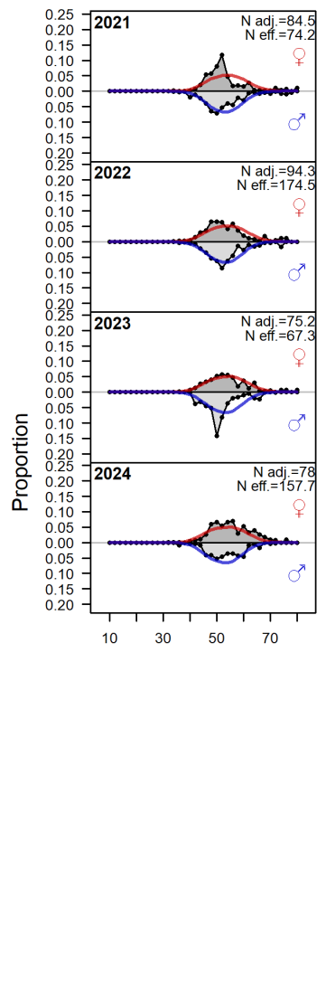
Figure 72: Observed (gray density plot) and expected (density lines by sex) length compositions by year for the non-trawl fishery in years available between 2021-2024. 'N adj.' is the input sample size after data-weighting adjustment. N eff. is the calculated effective sample size used in the McAllister-Ianelli tuning method.
