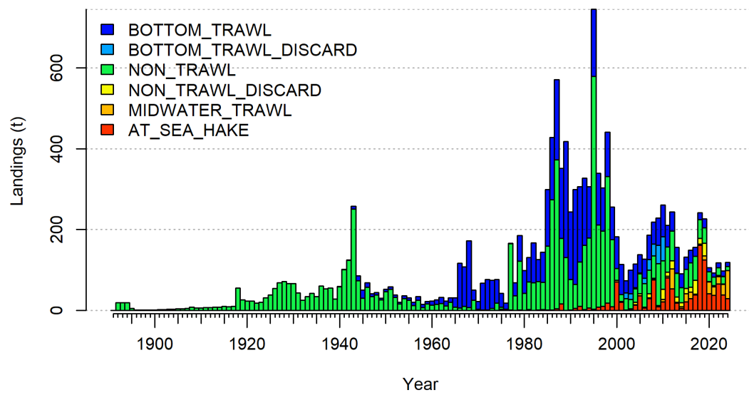
Figure 6: Landings by fleet.
