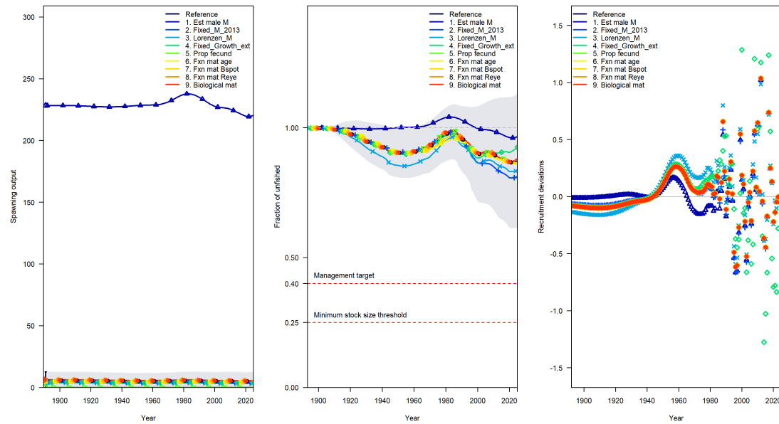
Figure 158: Comparison of spawning output (left panel), relative stock status (middle panel) and recruitment estimation (right panel) for models under different natural mortality, growth and reproductive biology scenarios.
