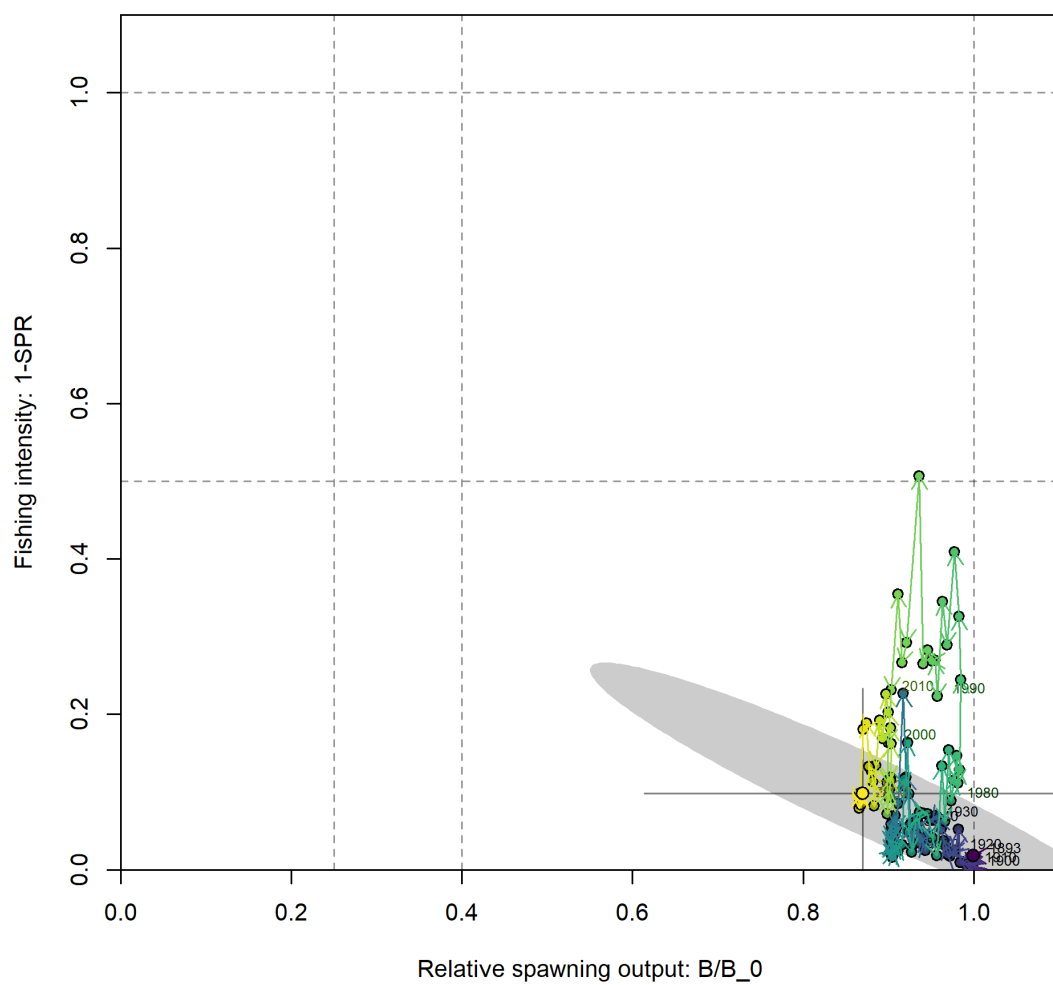
Figure 176: Phase plot of fishing intensity versus fraction unfished.
