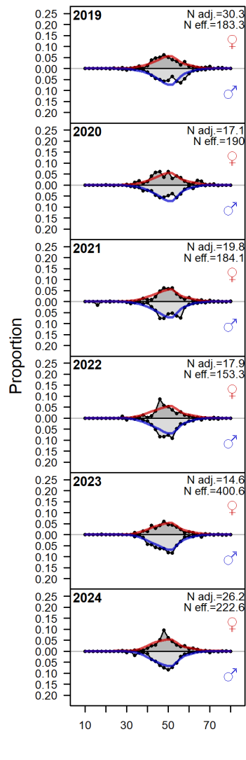
Figure 69: Observed (gray density plot) and expected (density lines by sex) length compositions by year for the bottom trawl fishery in years available between 2019-2024. 'N adj.' is the input sample size after data-weighting adjustment. N eff. is the calculated effective sample size used in the McAllister-Ianelli tuning method.
