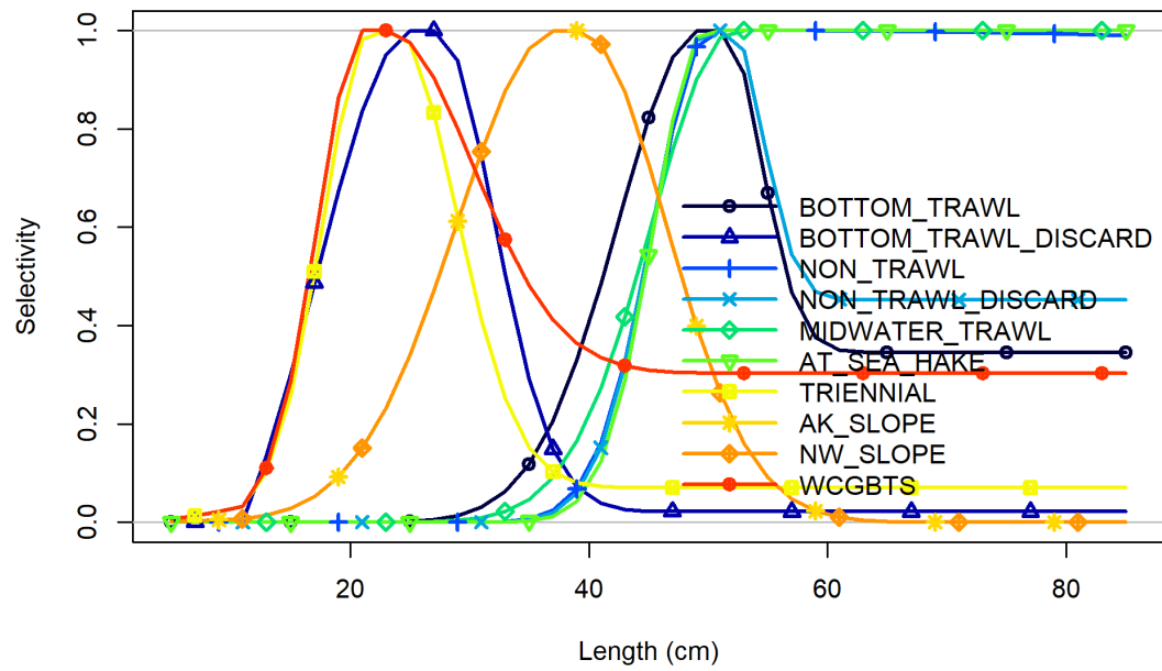
Figure 132: Ending selectivity at length for each fishery and survey.
