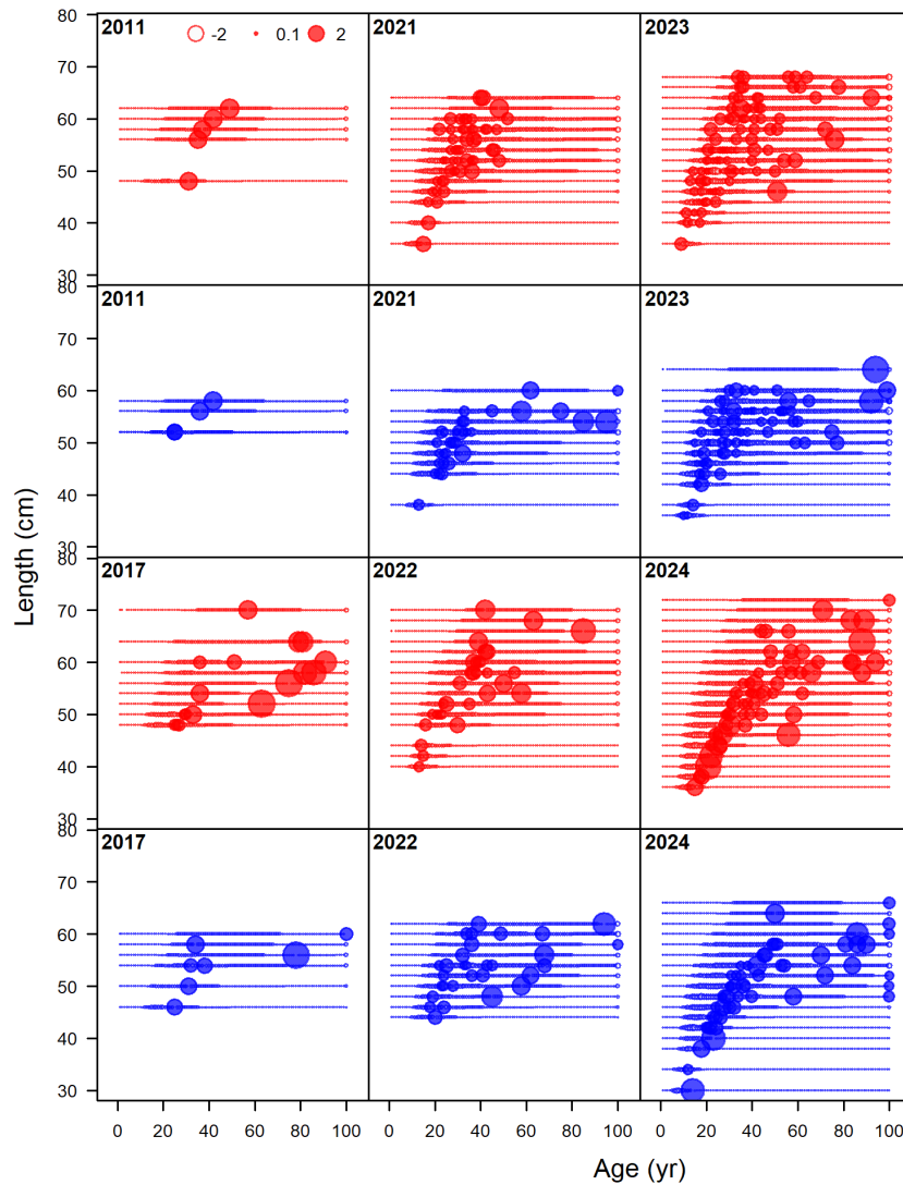
Figure 94: Pearson residuals of conditional age at length fits for the midwater trawl fishery. Closed bubble are positive residuals (observed > expected) and open bubbles are negative residuals (observed < expected).
