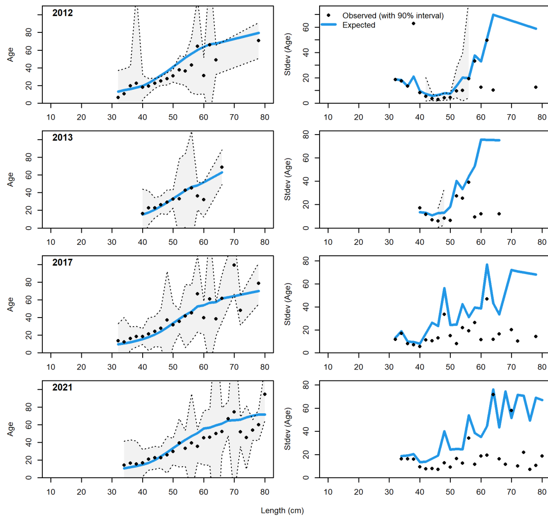
Figure 109: Conditional age at length plot showing mean age (left panels) and standard deviation (right panels) for the non-trawl fishery in years 2012-2021. The CIs are 90% based on adding 1.64 SE of mean to the data for the left panels and the standard error of mean age at length (obs. and exp.) with 90% CIs based on the chi-square distribution.
