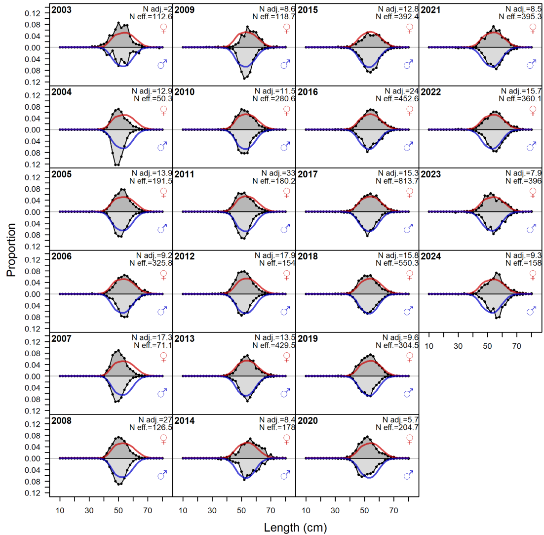
Figure 75: Observed (gray density plot) and expected (density lines by sex) length compositions by year for the at-sea-hake fishery in years available between 2003-2024. 'N adj.' is the input sample size after data-weighting adjustment. N eff. is the calculated effective sample size used in the McAllister-Ianelli tuning method.
