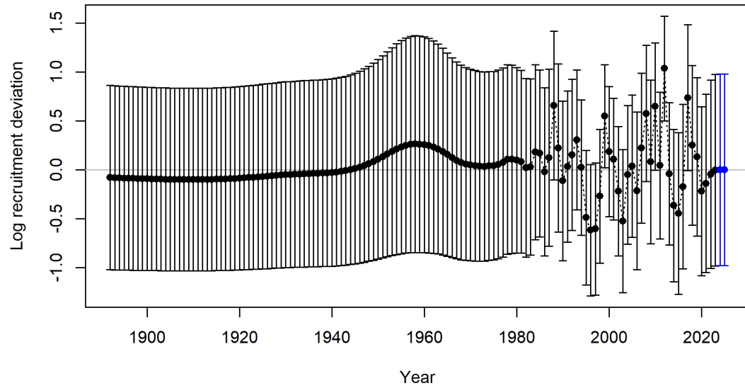
Figure 139: Estimated time series of recruitment deviations for the base model.
