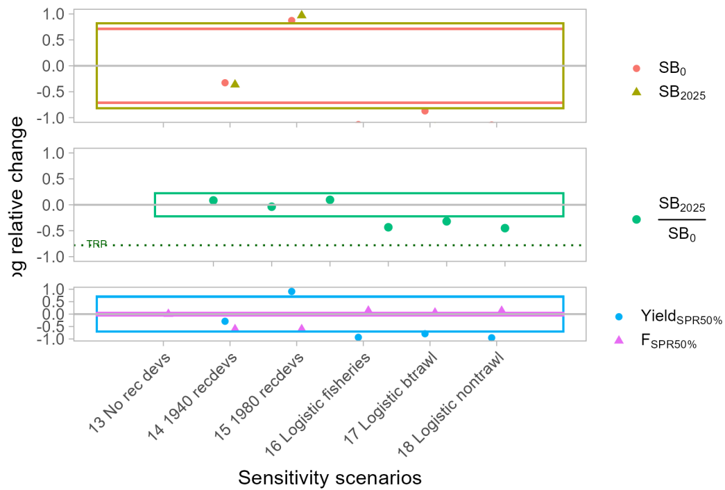
Figure 162: Log relative change ( \log((\text{Model\_sensi} - \text{Model\_ref}) / \text{Model\_ref}) ) in recruitment and selectivity scenarios for 5 derived quantities. Colored boxes indicate 95 percent confidence interval of the reference model. See ‘Sensitivity Analysis’ section for more details on each scenario.
