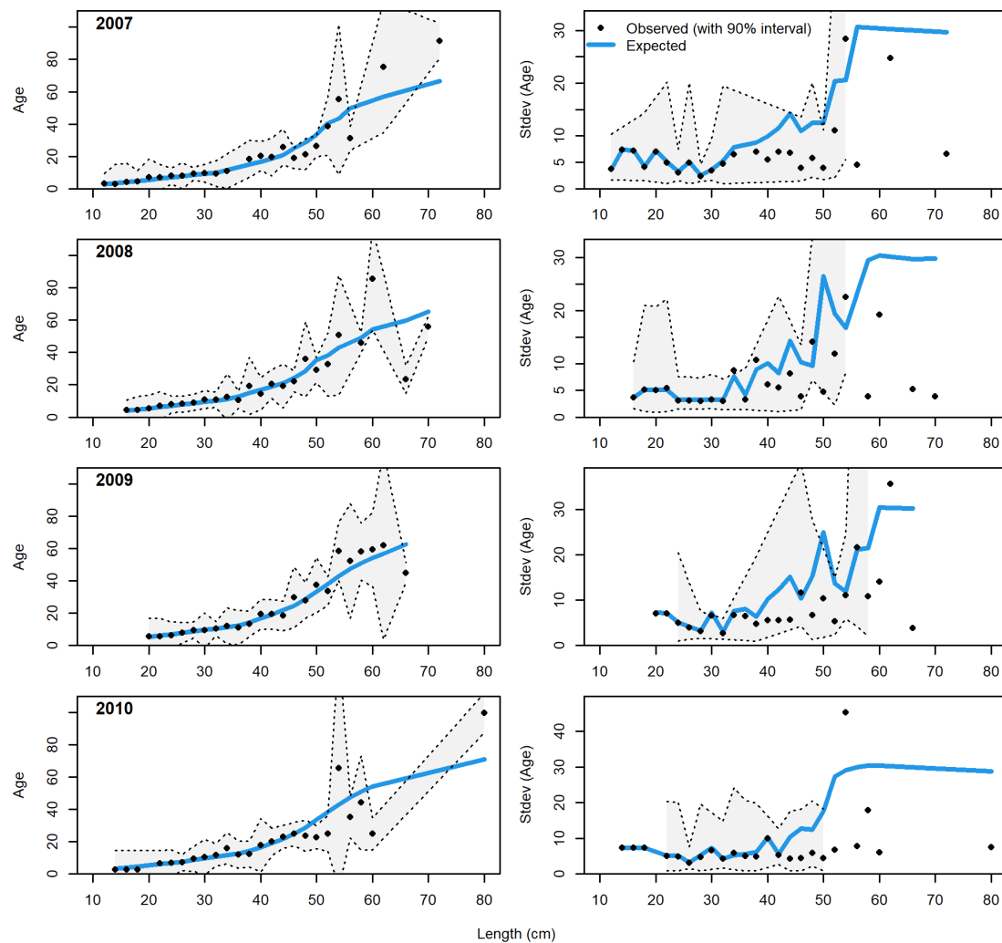
Figure 117: Conditional age at length plot showing mean age (left panels) and standard deviation (right panels) for the West Coast Groundfish Bottom Trawl survey in years 2007-2010. The CIs are 90% based on adding 1.64 SE of mean to the data for the left panels and the standard error of mean age at length (obs. and exp.) with 90% CIs based on the chi-square distribution.
