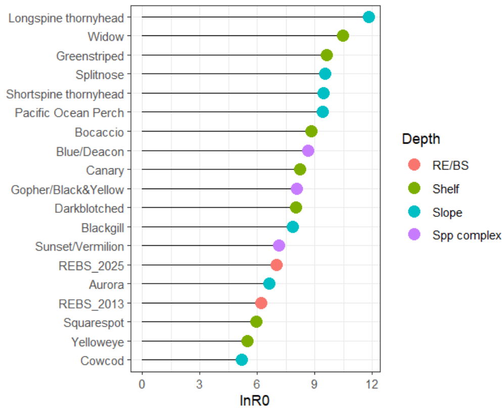
Figure 136: Estimated unfished recruitment ( \ln R_0 ) for several assessed shelf and slope rockfishes.
