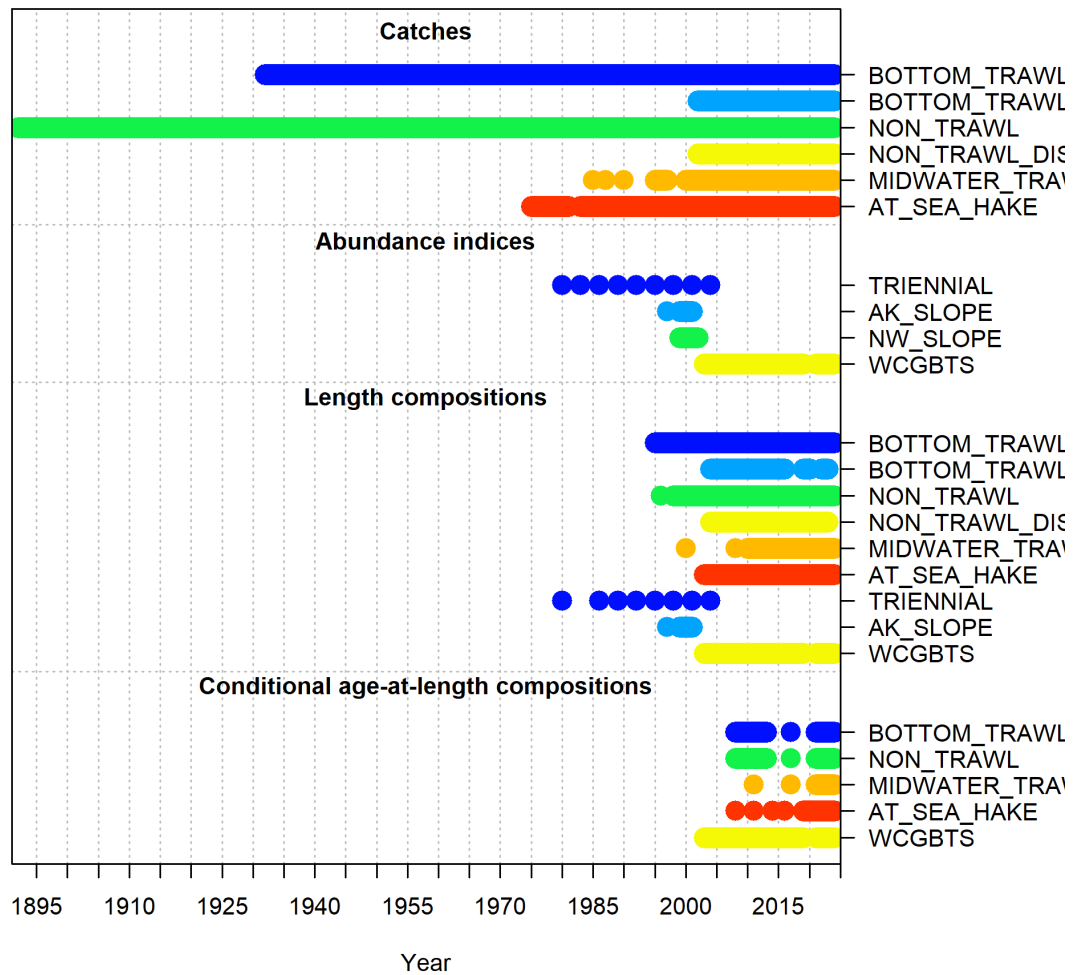
Figure 5: Data used in the base model.
