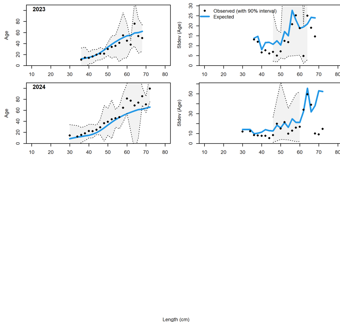
Figure 112: Conditional age at length plot showing mean age (left panels) and standard deviation (right panels) for the non-trawl fishery in years 2023-2024. The CIs are 90% based on adding 1.64 SE of mean to the data for the left panels and the standard error of mean age at length (obs. and exp.) with 90% CIs based on the chi-square distribution.
