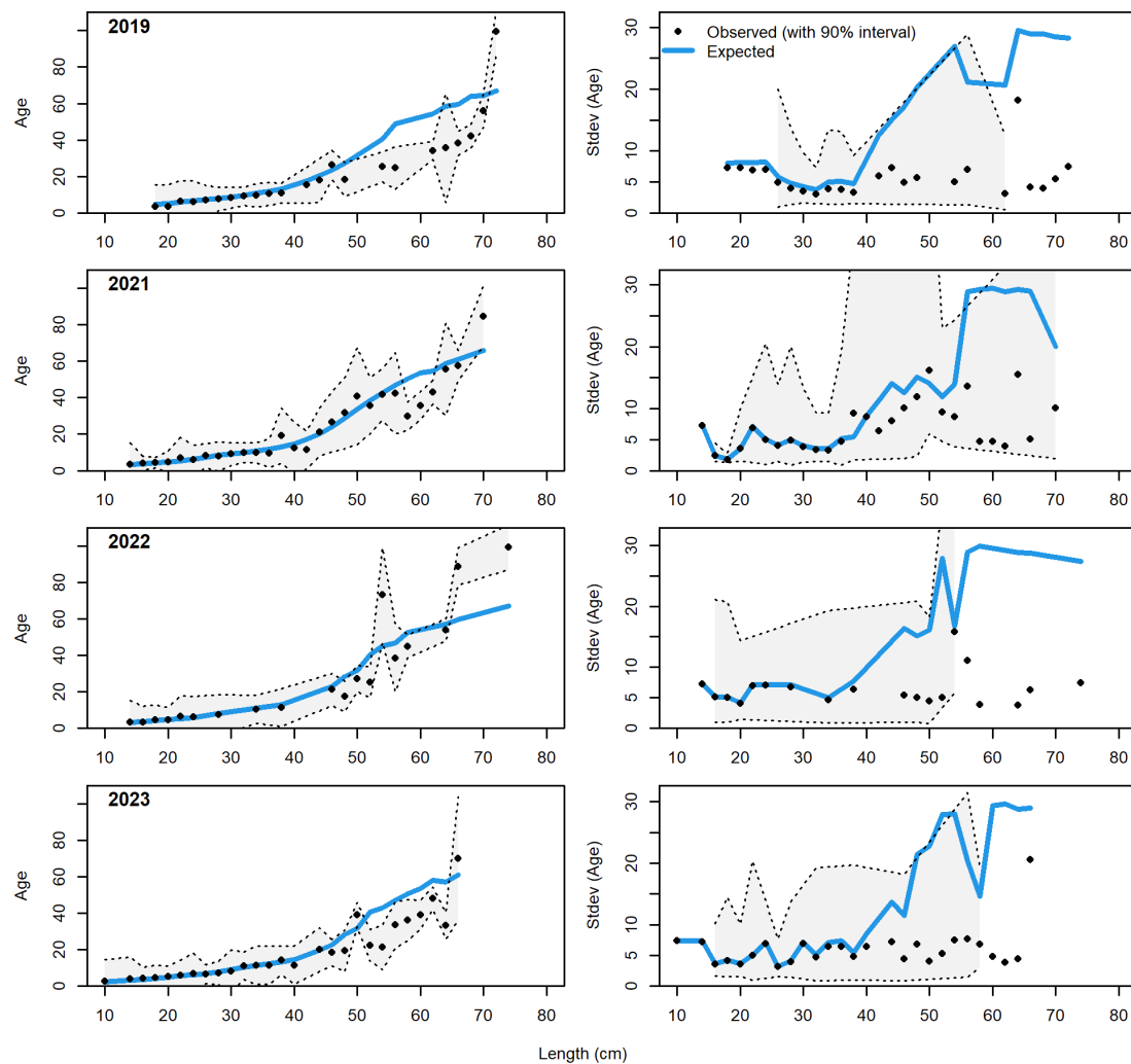
Figure 120: Conditional age at length plot showing mean age (left panels) and standard deviation (right panels) for the West Coast Groundfish Bottom Trawl survey in years 2019-2023. The CIs are 90% based on adding 1.64 SE of mean to the data for the left panels and the standard error of mean age at length (obs. and exp.) with 90% CIs based on the chi-square distribution.
