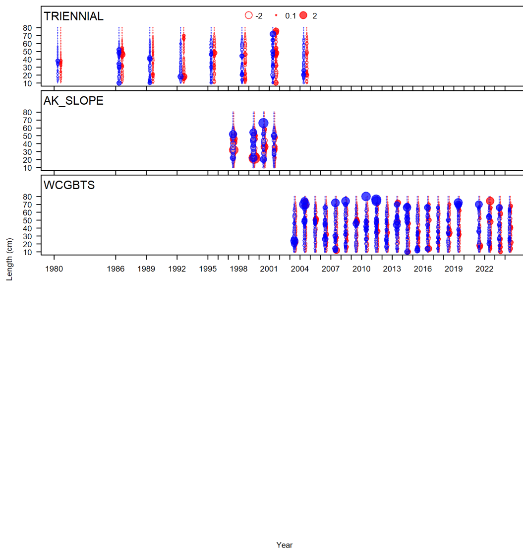
Figure 80: Pearson residuals of length fits for each survey. Closed bubble are positive residuals (observed > expected) and open bubbles are negative residuals (observed < expected).
