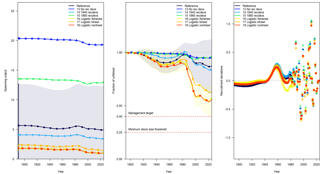
Figure 161: Comparison of spawning output (left panel), relative stock status (middle panel) and recruitment estimation (right panel) for models under different recruitment and selectivity scenarios.
