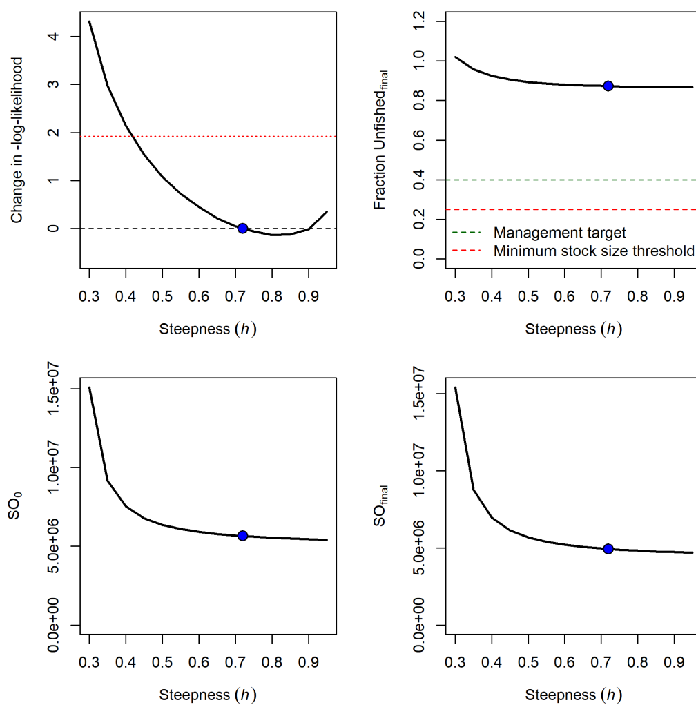
Figure 166: Steepness ( h ) likelihood profile (change in the negative log-likelihood across a range of h values) and derived quantities. Red line in the top left figure indicates the significance level in likelihood difference.
