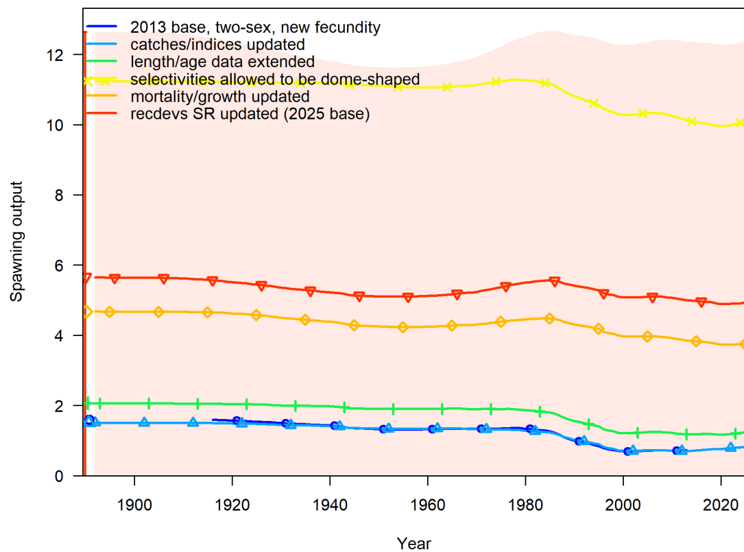
Figure 61: Time series of estimated spawning output for bridging analysis.
