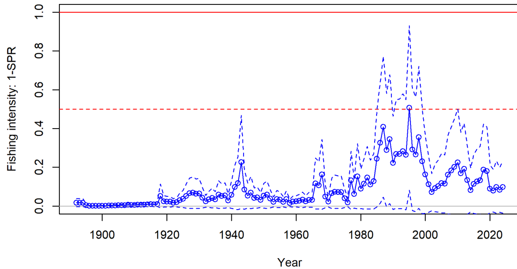
Figure 174: Estimated time series of the fishing intensity ( 1 - \text{SPR} ), where SPR is the spawning potential ratio, with approximate 95% asymptotic intervals. The horizontal line at 0.5 corresponds to \text{SPR} = 0.5 , the management reference point. The horizontal line at 1.0 corresponds to \text{SPR} = 0 (all spawning fish removed from the population).
