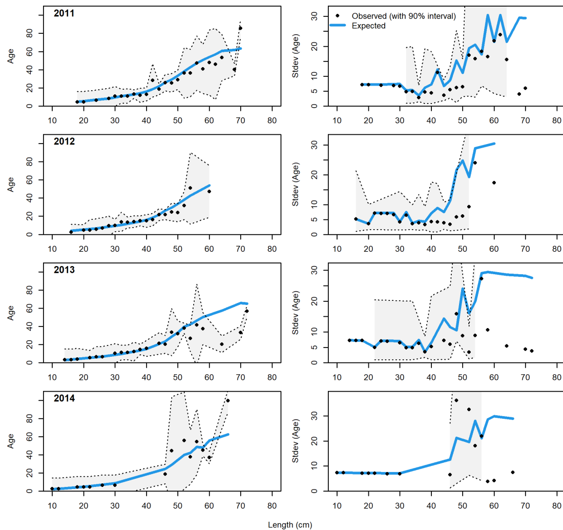
Figure 118: Conditional age at length plot showing mean age (left panels) and standard deviation (right panels) for the West Coast Groundfish Bottom Trawl survey in years 2011-2014. The CIs are 90% based on adding 1.64 SE of mean to the data for the left panels and the standard error of mean age at length (obs. and exp.) with 90% CIs based on the chi-square distribution.
