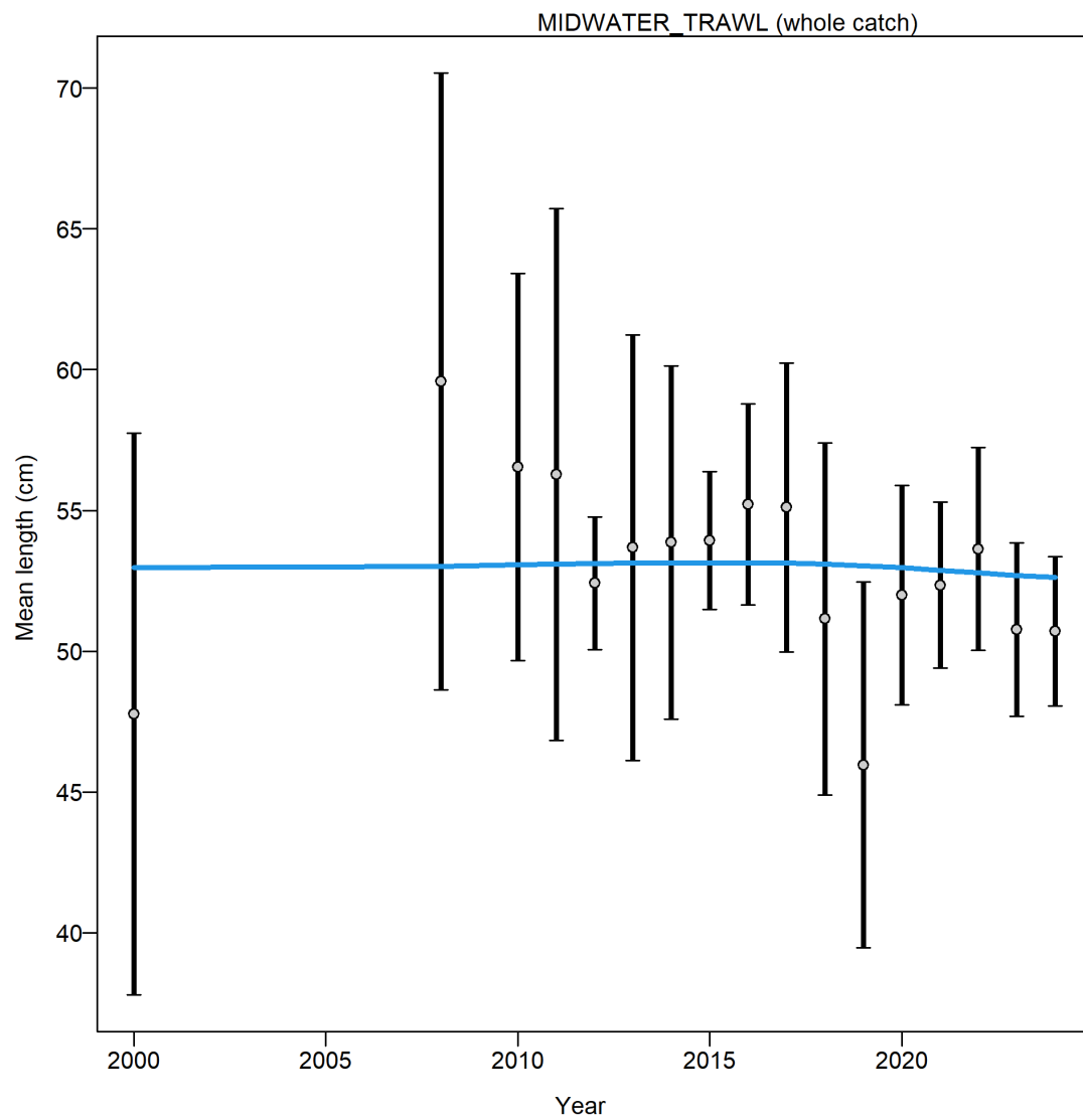
Figure 85: Mean length (cm) index from the midwater trawl fishery with 95 percent confidence intervals based on sample sizes and data weighting.
