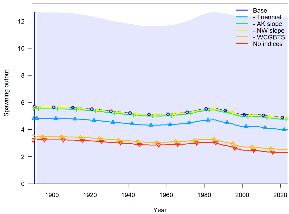
Figure 145: Spawning output (millions of eggs) across data removal sensitivities (indices).
