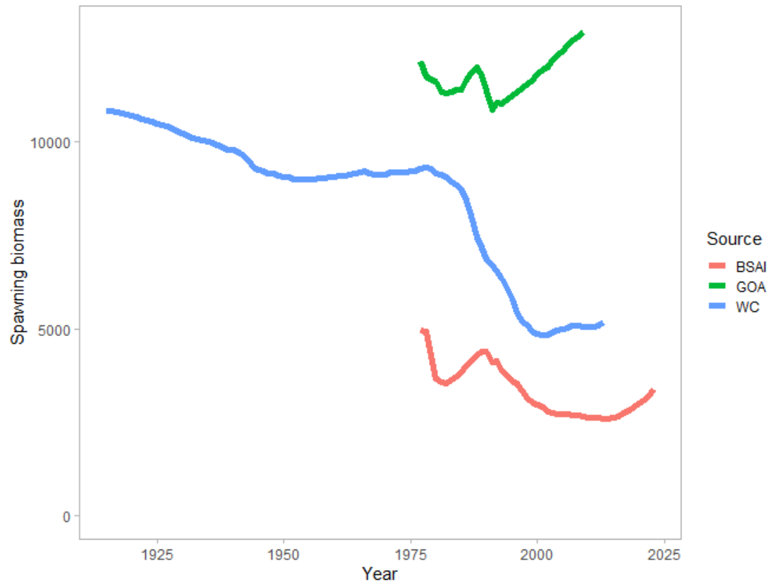
Figure 3: Estimates of spawning biomass (current spawning output/unfished spawning output) for the Rougheye/Blackspotted rockfish complex from the two most recent Alaska (Bering Sea/Aleutian Islands (BSAI) and Gulf of Alaska (GOA)) and the 2013 U.S. west coast stock assessment.
