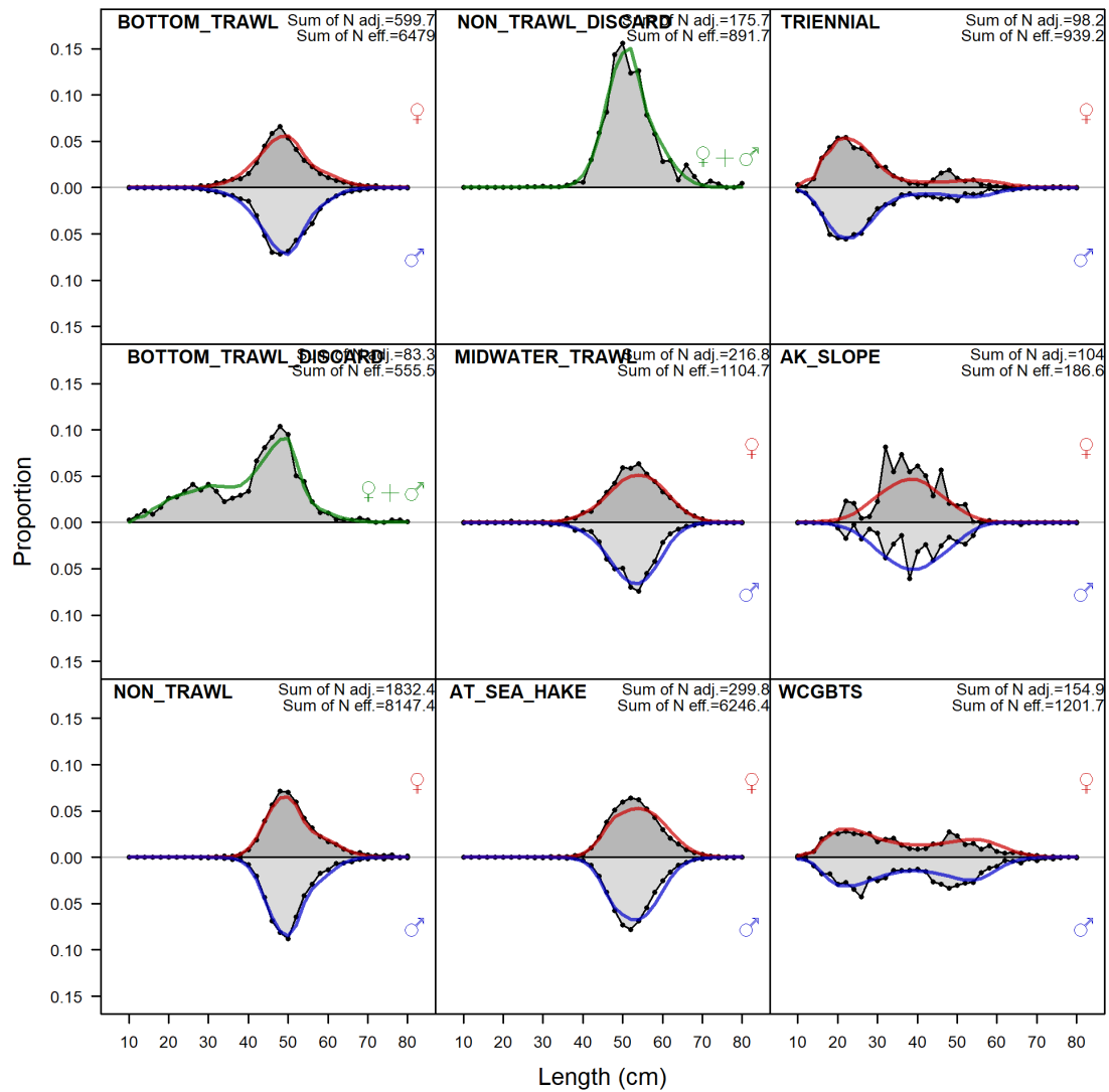
Figure 67: Aggregated length (cm) compositions over all years.
