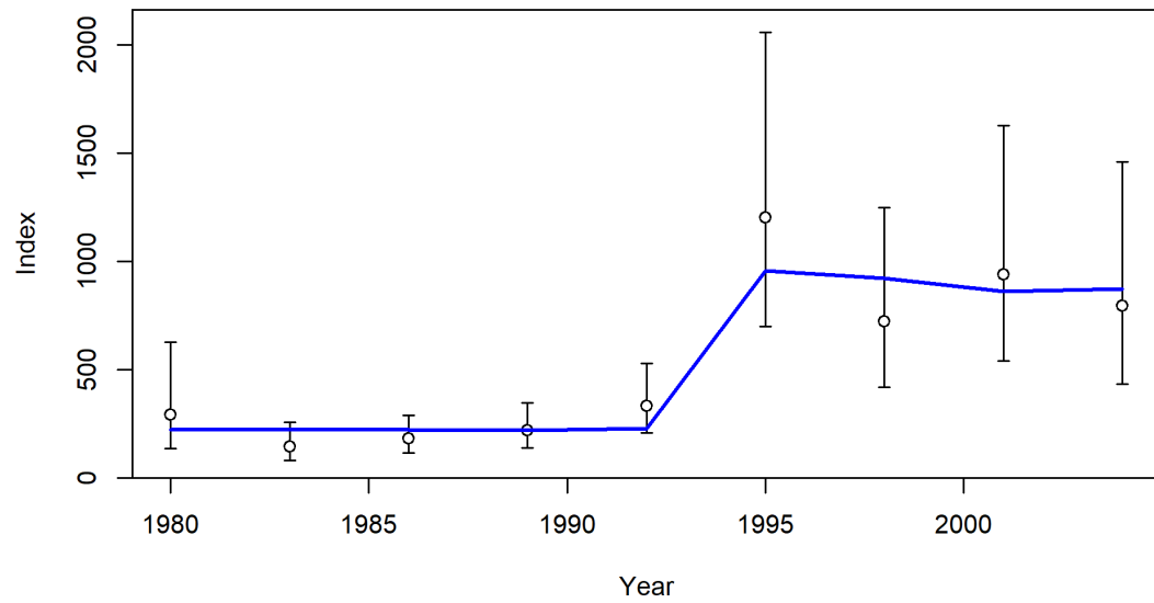
Figure 127: Fit to index data for Triennial survey. Lines indicate 95% uncertainty interval around index values based on the assumption of lognormal error.
