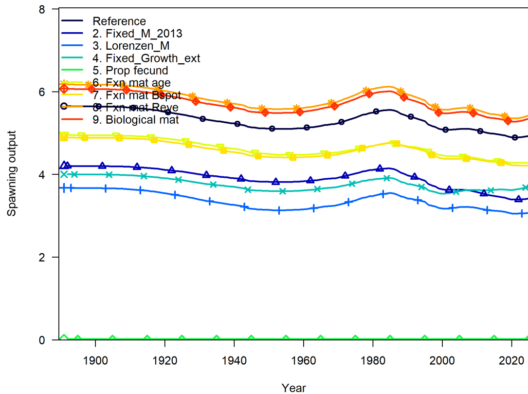
Figure 160: Comparison of spawning output for models under different natural mortality, growth and reproductive biology scenarios. This comparison excludes the model estimating natural mortality, as the scale goes extremely high.
