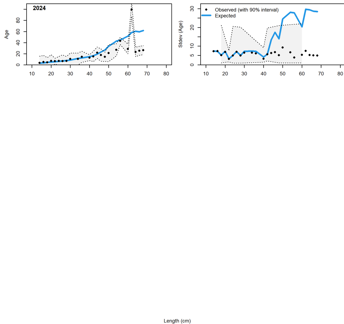
Figure 121: Conditional age at length plot showing mean age (left panels) and standard deviation (right panels) for the West Coast Groundfish Bottom Trawl survey in 2024. The CIs are 90% based on adding 1.64 SE of mean to the data for the left panels and the standard error of mean age at length (obs. and exp.) with 90% CIs based on the chi-square distribution.
