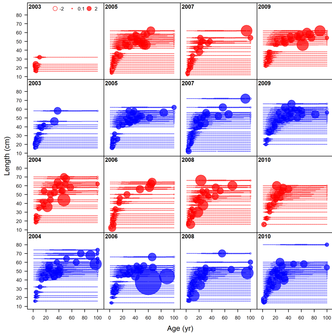
Figure 97: Pearson residuals of conditional age at length fits for the West Coast Groundfish Bottom Trawl survey in the years 2003-2010. Closed bubble are positive residuals (observed > expected) and open bubbles are negative residuals (observed < expected).
