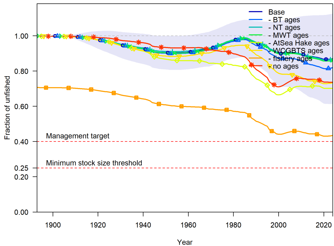
Figure 152: Relative spawning output (fraction unfished) across data removal sensitivities (age compositions by fleet).
