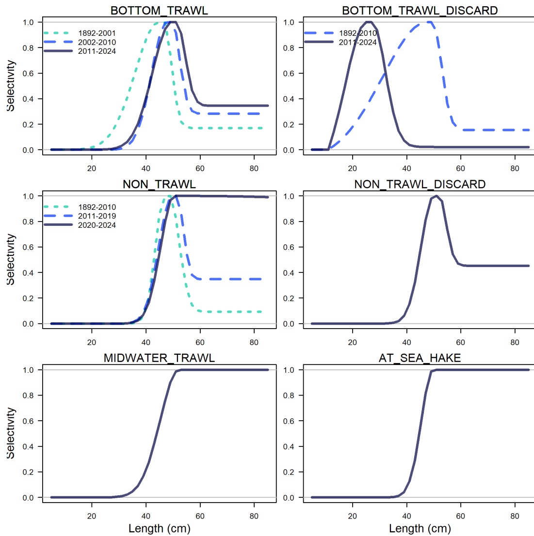
Figure 133: Time-varying selectivity for fishery fleets with time blocks.
