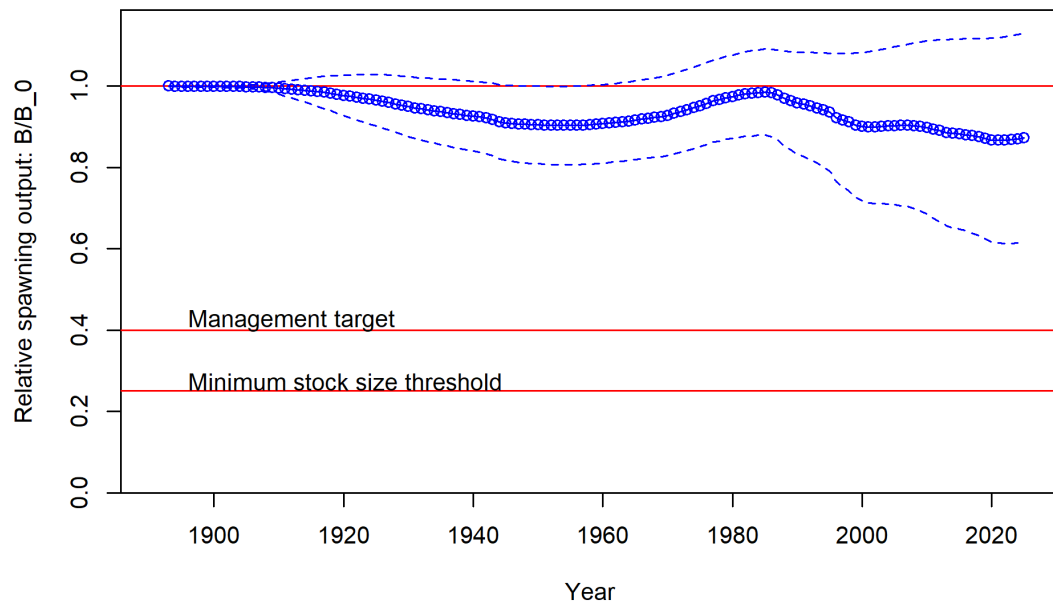
Figure 138: Estimated time series of fraction of unfished spawning output for the reference model.
