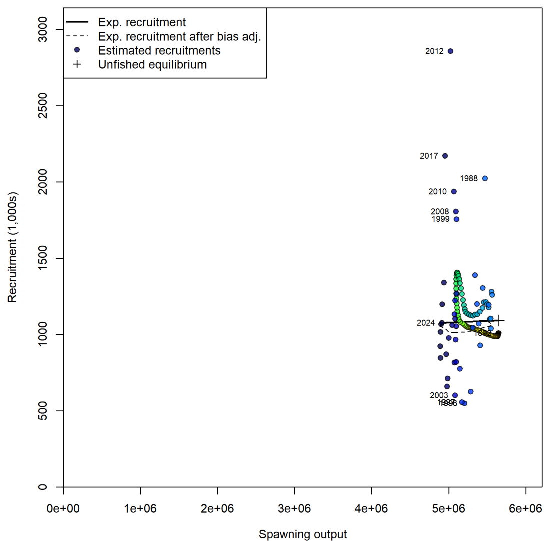
Figure 142: Stock-recruit curve with labels on first, last, and years with (log) deviations > 0.5 . Point colors indicate year, with warmer colors indicating earlier years and cooler colors in showing later years.
