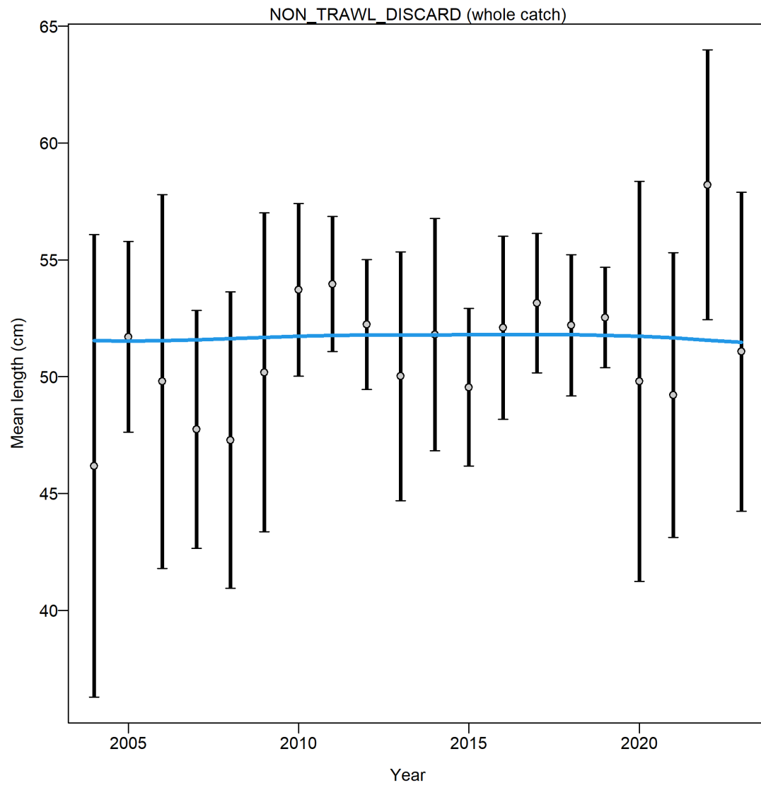
Figure 84: Mean length (cm) index from the non-trawl discard fishery with 95 percent confidence intervals based on sample sizes and data weighting.
