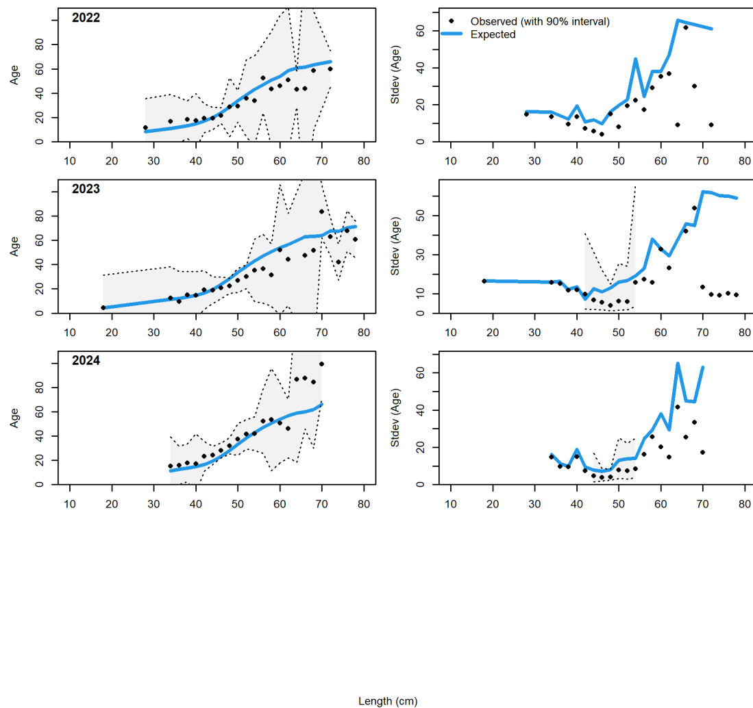
Figure 107: Conditional age at length plot showing mean age (left panels) and standard deviation (right panels) for the bottom trawl fishery in years 2022-2024. The CIs are 90% based on adding 1.64 SE of mean to the data for the left panels and the standard error of mean age at length (obs. and exp.) with 90% CIs based on the chi-square distribution.
