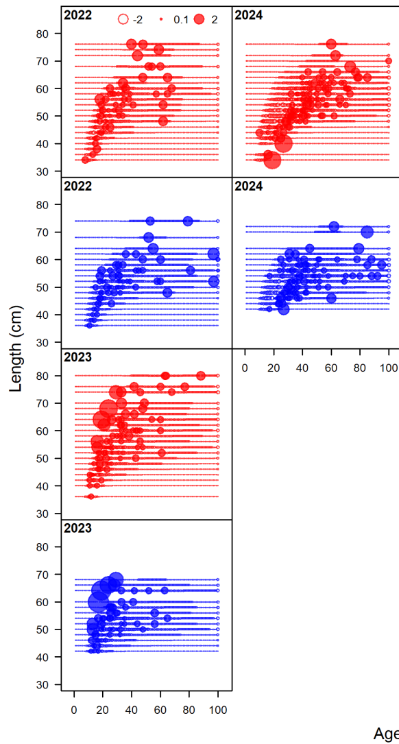
Figure 93: Pearson residuals of conditional age at length fits for the non-trawl fishery in the years 2022-2024. Closed bubble are positive residuals (observed > expected) and open bubbles are negative residuals (observed < expected).
