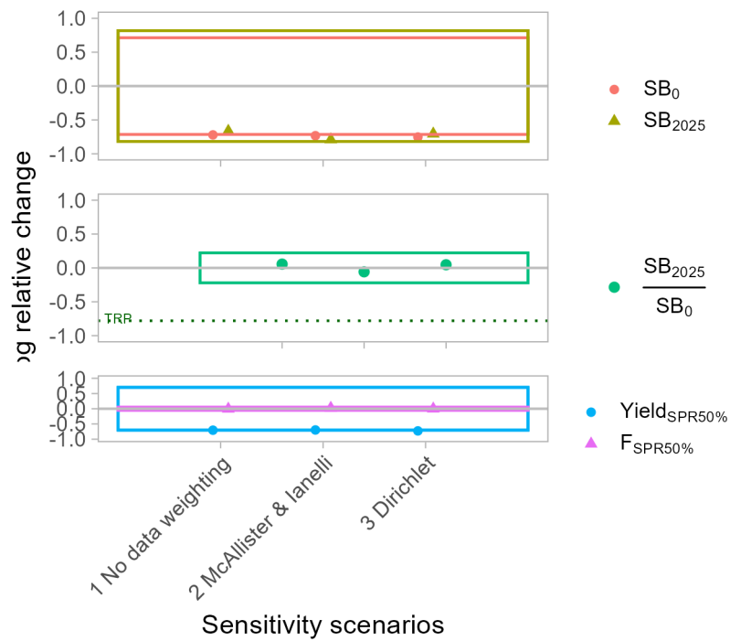
Figure 155: Log relative change ( \log((\text{Model\_sensi}-\text{Model\_ref})/\text{Model\_ref})) in data weighting treatment for 5 derived quantities. Colored boxes indicate 95 percent confidence interval of the reference model. See ‘Sensitivity Analysis’ section for more details on each scenario.
