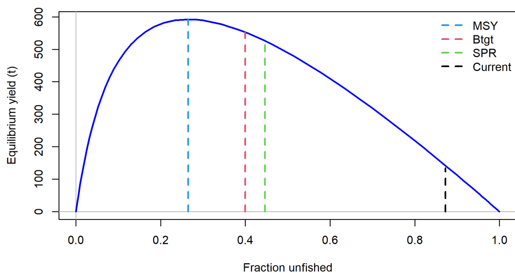
Figure 175: Equilibrium yield curve for the base case model. Values are based on the most recent fishery selectivities and retention curves and with steepness fixed at 0.72.
