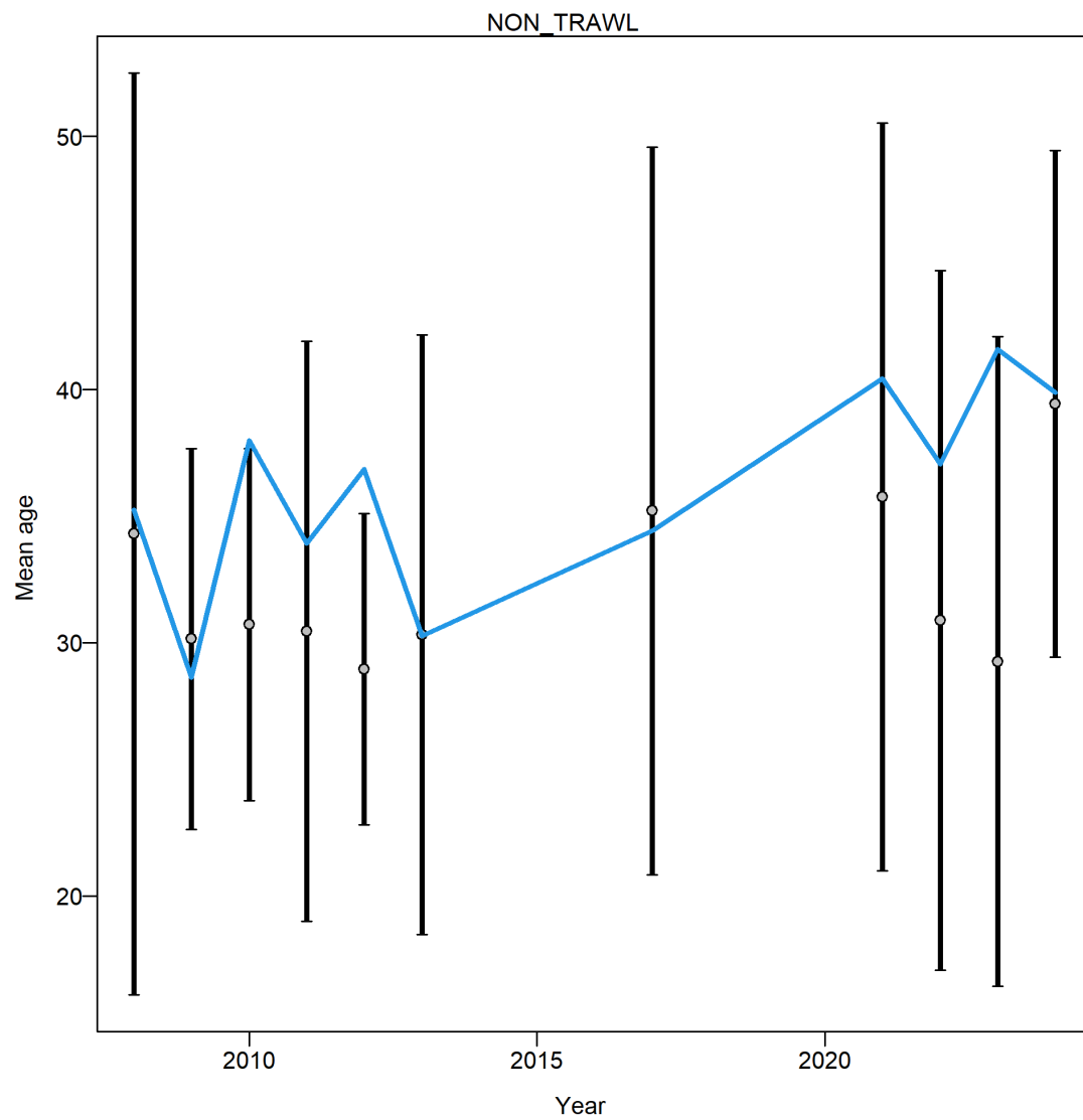
Figure 101: Mean age from conditional age-at-length data for the non-trawl fishery with 95% confidence intervals based on current samples sizes and data weighting.
