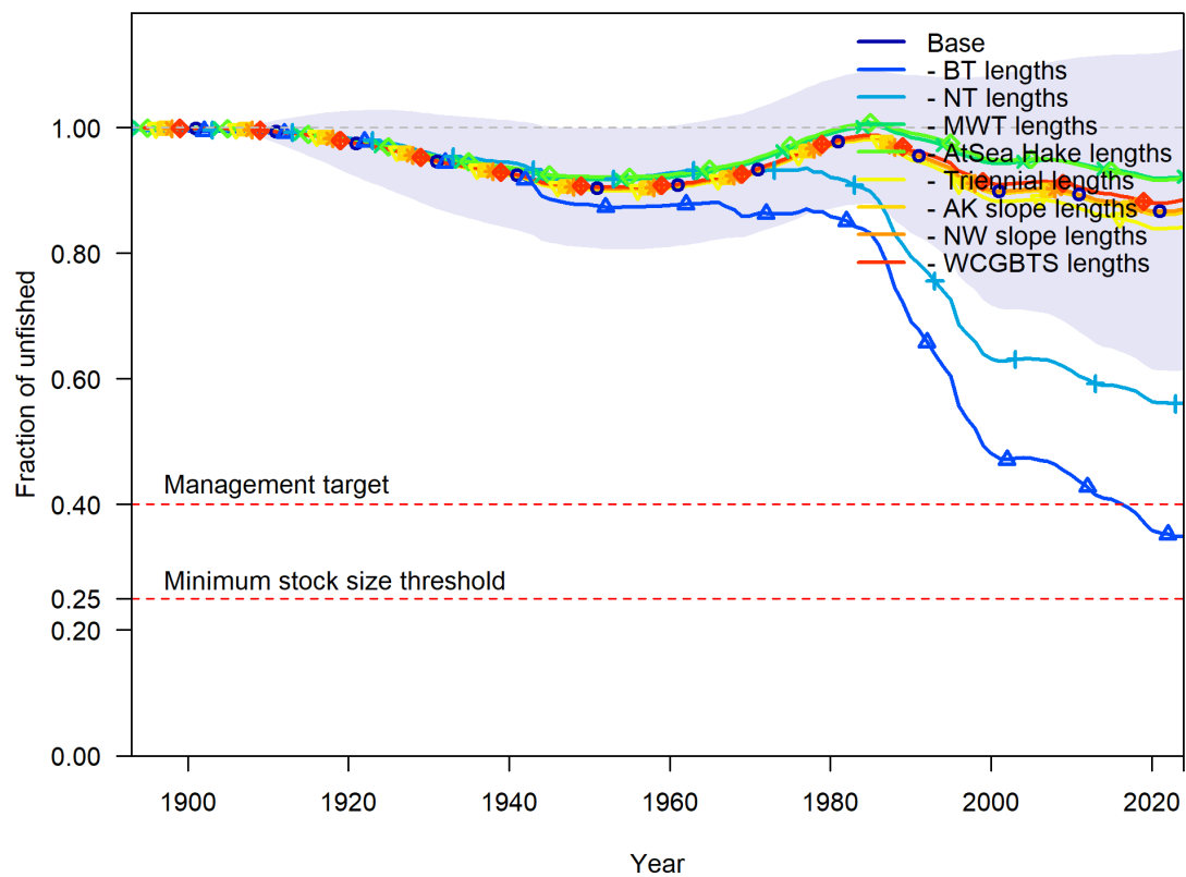
Figure 148: Relative spawning output (fraction unfished) across data removal sensitivities (length compositions by fleet).
