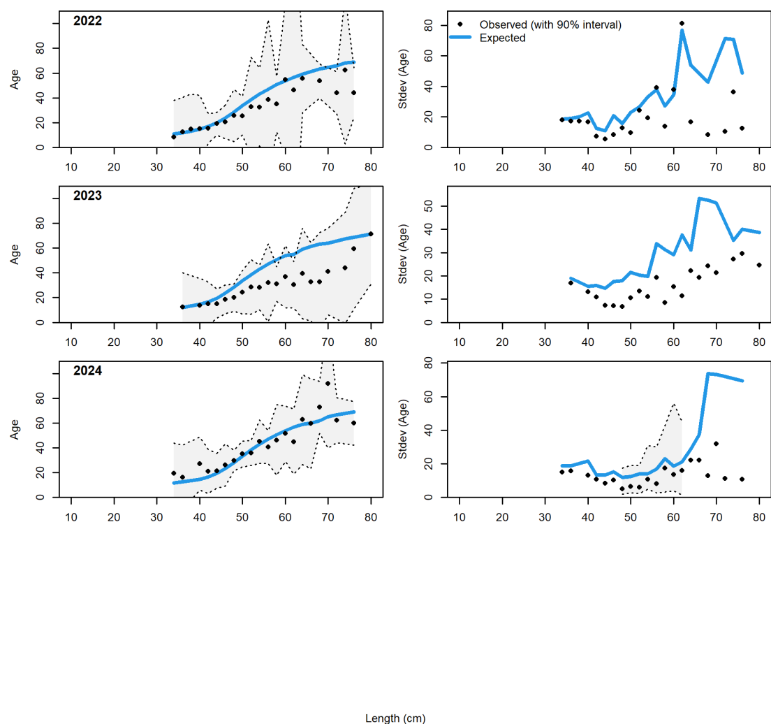
Figure 110: Conditional age at length plot showing mean age (left panels) and standard deviation (right panels) for the non-trawl fishery in years 2022-2024. The CIs are 90% based on adding 1.64 SE of mean to the data for the left panels and the standard error of mean age at length (obs. and exp.) with 90% CIs based on the chi-square distribution.
