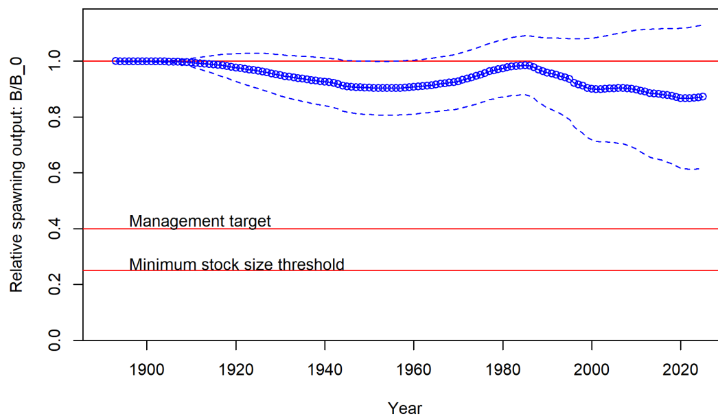
Figure 173: Estimated time series of fraction of unfished spawning output for the base model.
