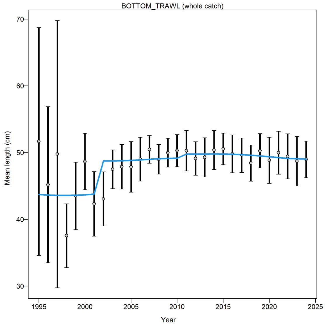
Figure 81: Mean length (cm) index from the bottom trawl fishery with 95 percent confidence intervals based on sample sizes and data weighting.
