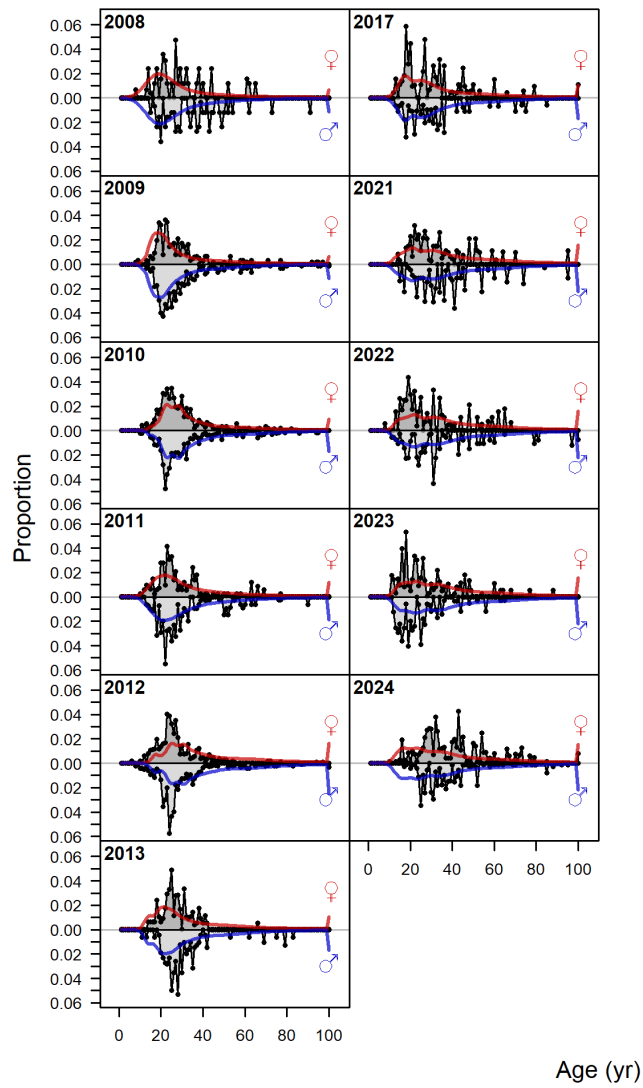
Figure 123: Realized fits (lines) to the marginal age composition data (density) for the non-trawl fishery.
