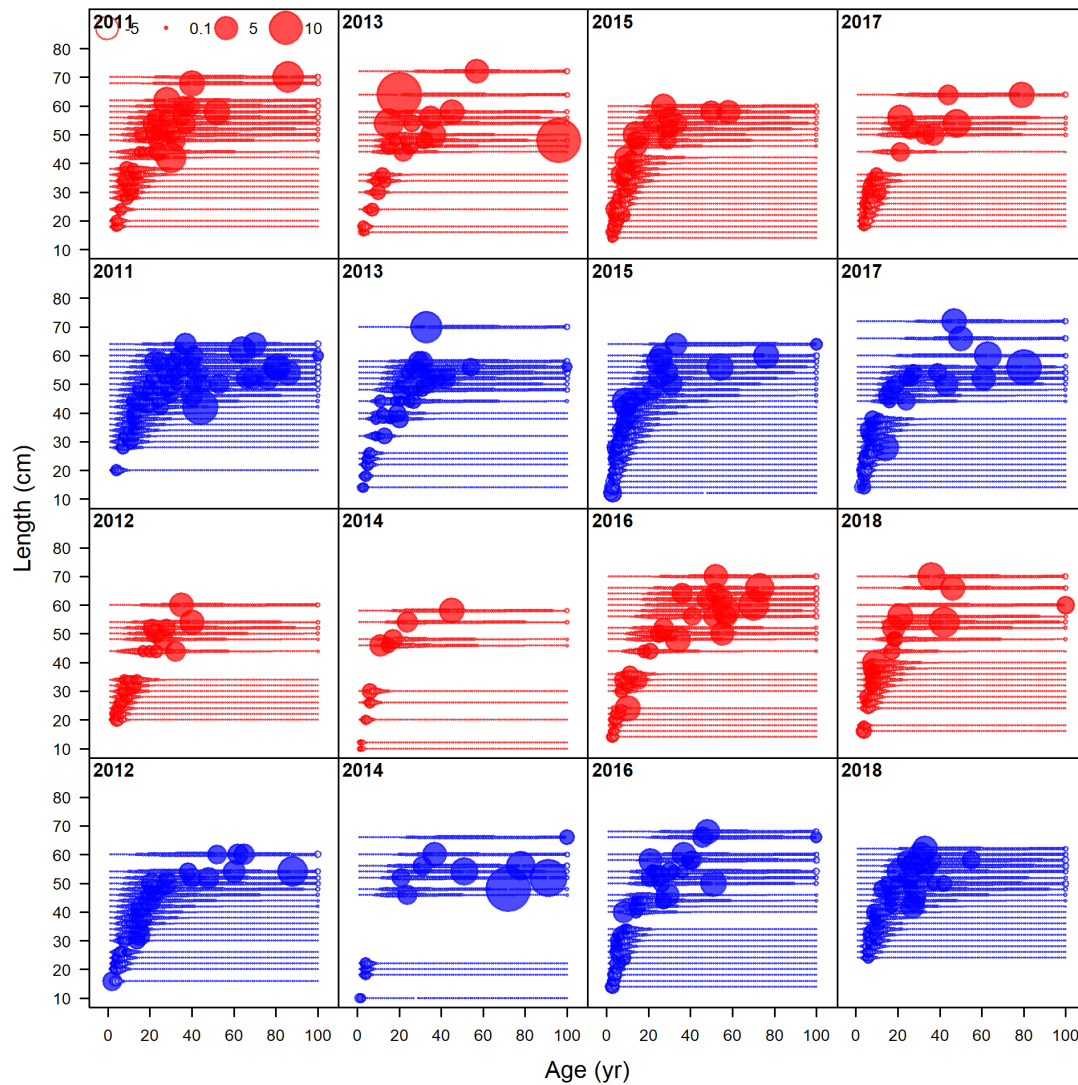
Figure 98: Pearson residuals of conditional age at length fits for the West Coast Groundfish Bottom Trawl survey in the years 2011-2018. Closed bubble are positive residuals (observed > expected) and open bubbles are negative residuals (observed < expected).
