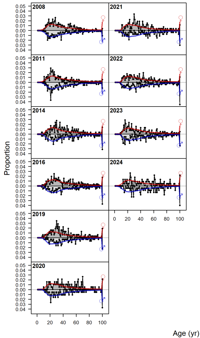
Figure 125: Realized fits (lines) to the marginal age composition data (density) for the at-sea-hake fishery.
