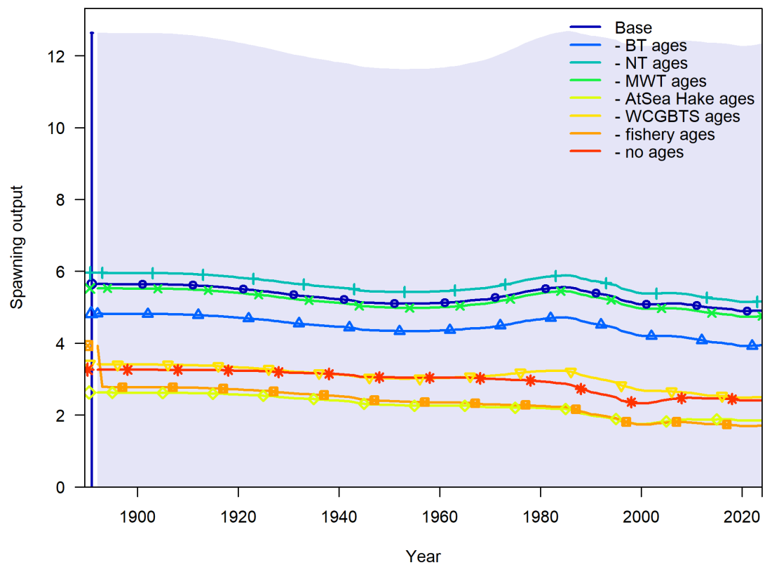
Figure 151: Spawning output (millions of eggs) across data removal sensitivities (age compositions by fleet).
