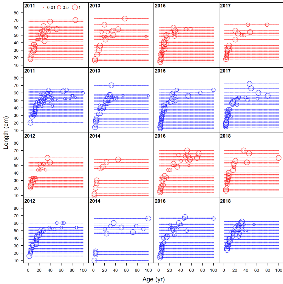
Figure 30: Conditional ages-at-length composition data for WCGBTS, continued.
