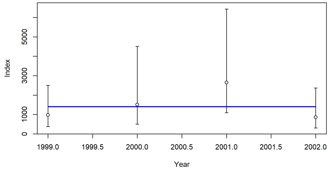
Figure 129: Fit to index data for Northwest Fisheries Science Center Slope survey. Lines indicate 95% uncertainty interval around index values based on the assumption of lognormal error.
