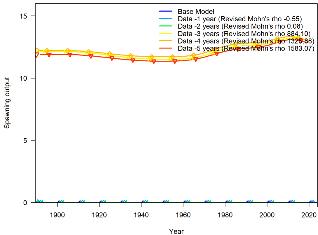
Figure 143: Change in the estimate of spawning output (millions of eggs) when the five most recent years of data area removed sequentially.
