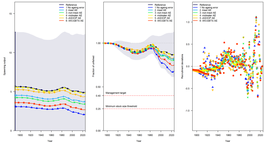
Figure 156: Comparison of spawning output (left panel), relative stock status (middle panel) and recruitment estimation (right panel) for models under different ageing error scenarios. The reference model uses ageing error matrices for all age sources.
