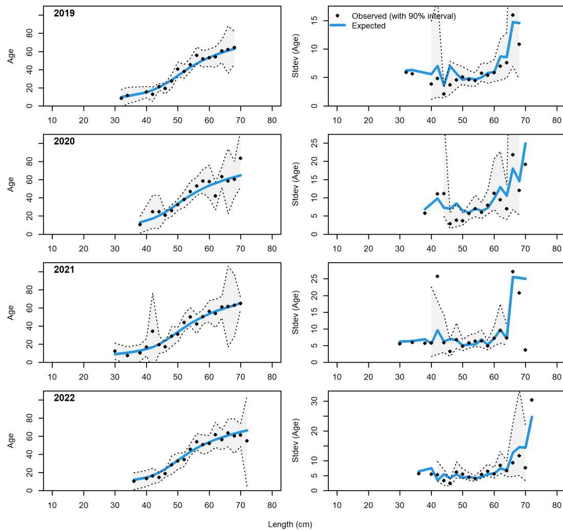
Figure 114: Conditional age at length plot showing mean age (left panels) and standard deviation (right panels) for the at-sea-hake fishery in years 2019-2022. The CIs are 90% based on adding 1.64 SE of mean to the data for the left panels and the standard error of mean age at length (obs. and exp.) with 90% CIs based on the chi-square distribution.
