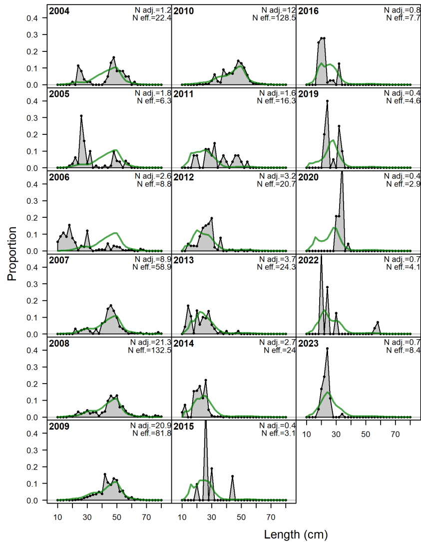
Figure 70: Observed (gray density plot) and expected (density lines) length compositions by year for the bottom trawl discard fishery in years available between 2004-2023. 'N adj.' is the input sample size after data-weighting adjustment. N eff. is the calculated effective sample size used in the McAllister-Ianelli tuning method.
