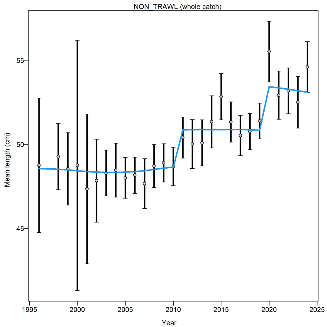
Figure 83: Mean length (cm) index from the non-trawl fishery with 95 percent confidence intervals based on sample sizes and data weighting.
