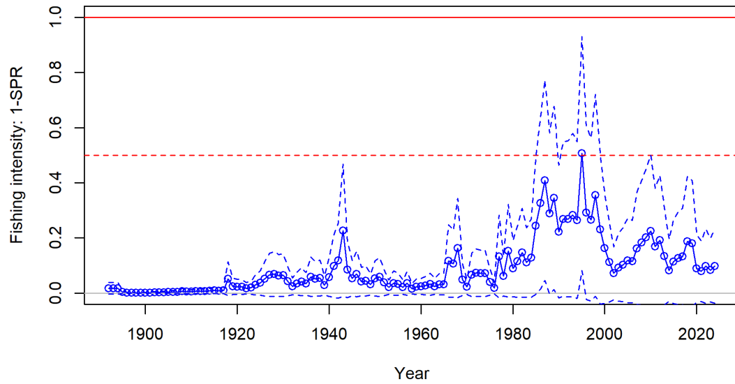
Figure 177: Estimated time series of fishing intensity for the base model.
