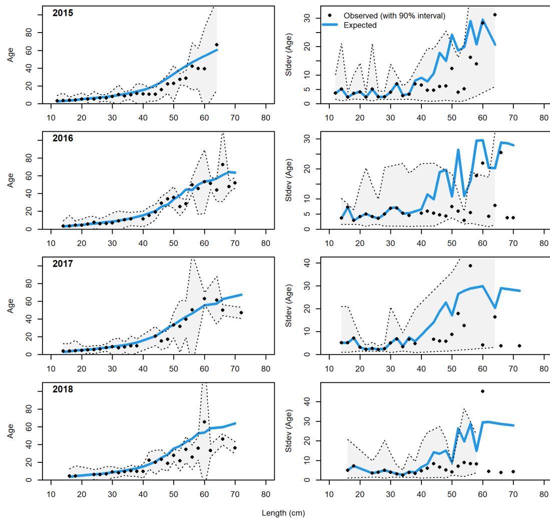
Figure 119: Conditional age at length plot showing mean age (left panels) and standard deviation (right panels) for the West Coast Groundfish Bottom Trawl survey in years 2015-2018. The CIs are 90% based on adding 1.64 SE of mean to the data for the left panels and the standard error of mean age at length (obs. and exp.) with 90% CIs based on the chi-square distribution.
