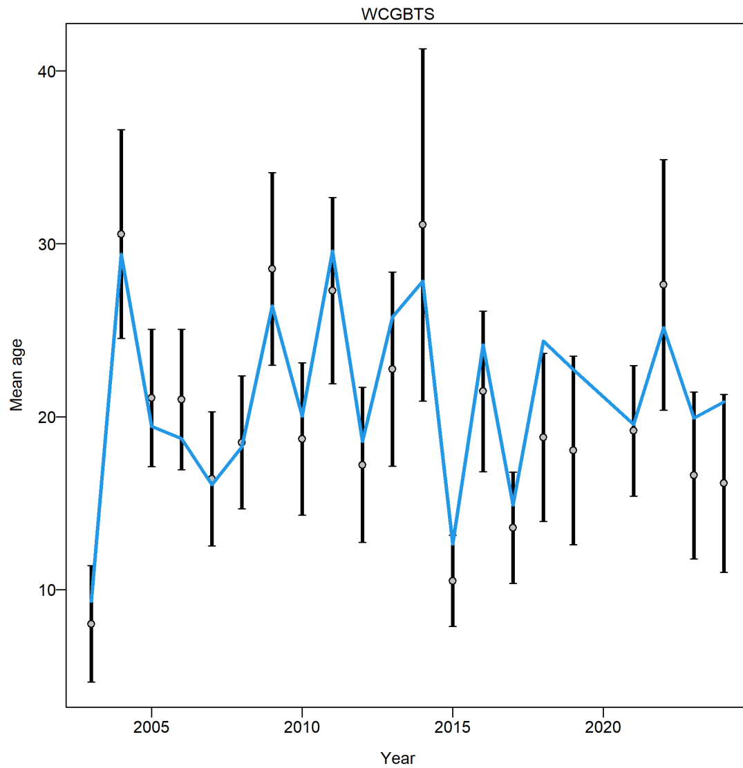
Figure 104: Mean age from conditional age-at-length data for the West Coast Groundfish Bottom Trawl survey with 95% confidence intervals based on current samples sizes and data weighting.
