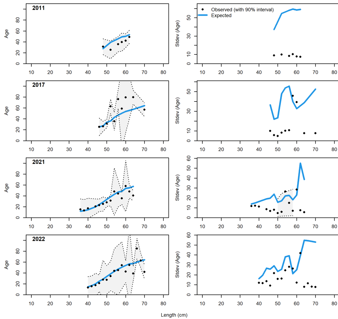
Figure 111: Conditional age at length plot showing mean age (left panels) and standard deviation (right panels) for the midwater trawl fishery in years 2011-2022. The CIs are 90% based on adding 1.64 SE of mean to the data for the left panels and the standard error of mean age at length (obs. and exp.) with 90% CIs based on the chi-square distribution.
