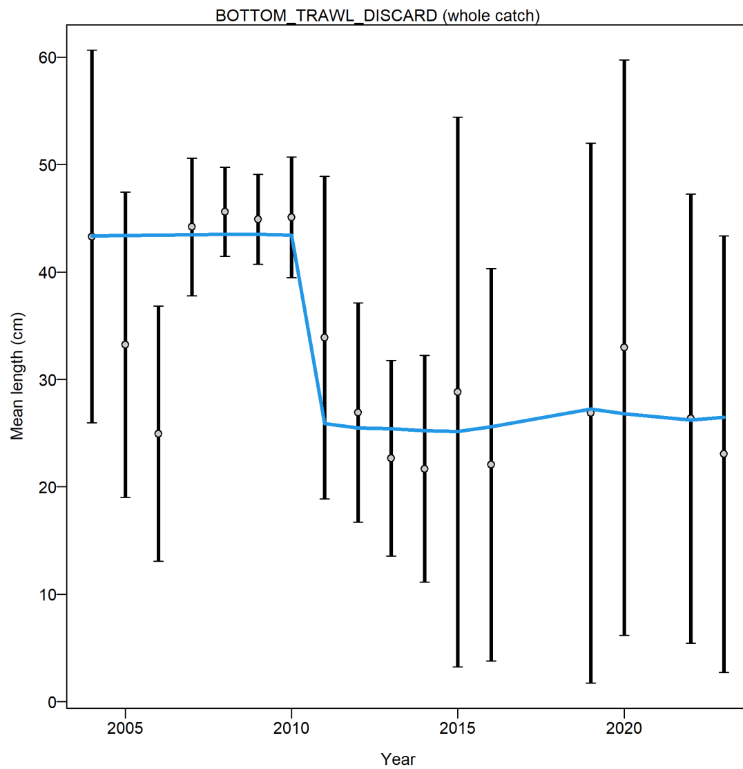
Figure 82: Mean length (cm) index from the bottom trawl discard fishery with 95 percent confidence intervals based on sample sizes and data weighting.
