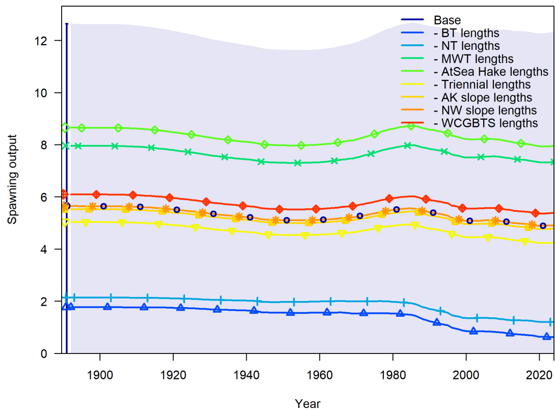
Figure 147: Spawning output (millions of eggs) across data removal sensitivities (length compositions by fleet).
