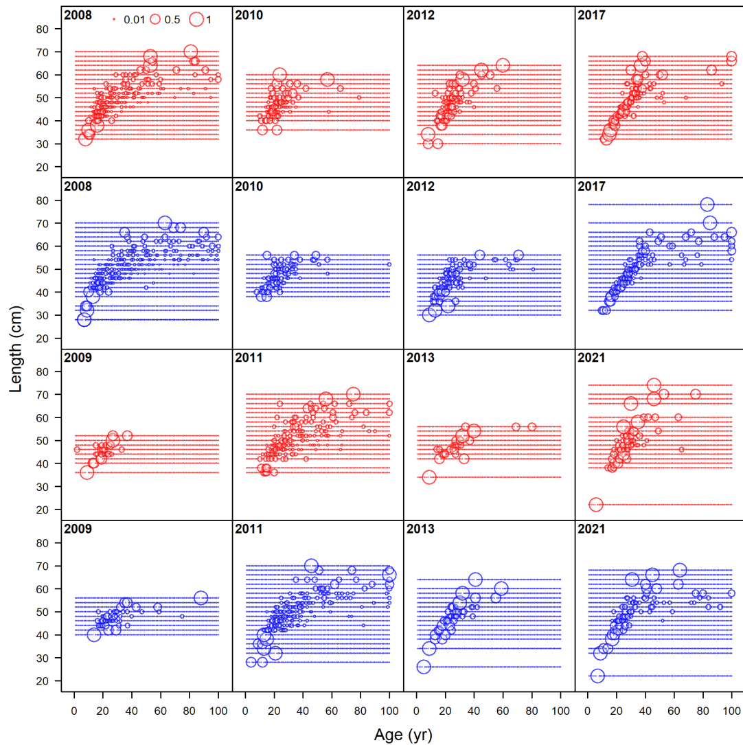
Figure 90: Pearson residuals of conditional age at length fits for the bottom trawl fishery in the years 2008-2021. Closed bubble are positive residuals (observed > expected) and open bubbles are negative residuals (observed < expected).
