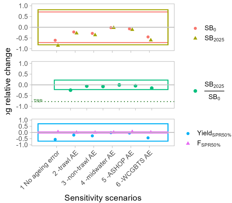
Figure 156: Log relative change ( \log((\text{Model\_sensi}-\text{Model\_ref})/\text{Model\_ref})) in ageing error scenarios for 5 derived quantities. Colored boxes indicate 95 percent confidence interval of the reference model. See ‘Sensitivity Analysis’ section for more details on each scenario.
