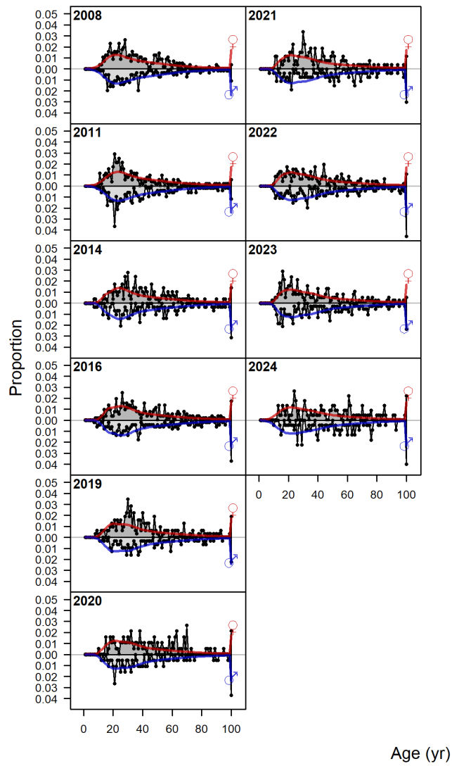
Figure 124: Realized fits (lines) to the marginal age composition data (density) for the at-sea-hake fishery.
