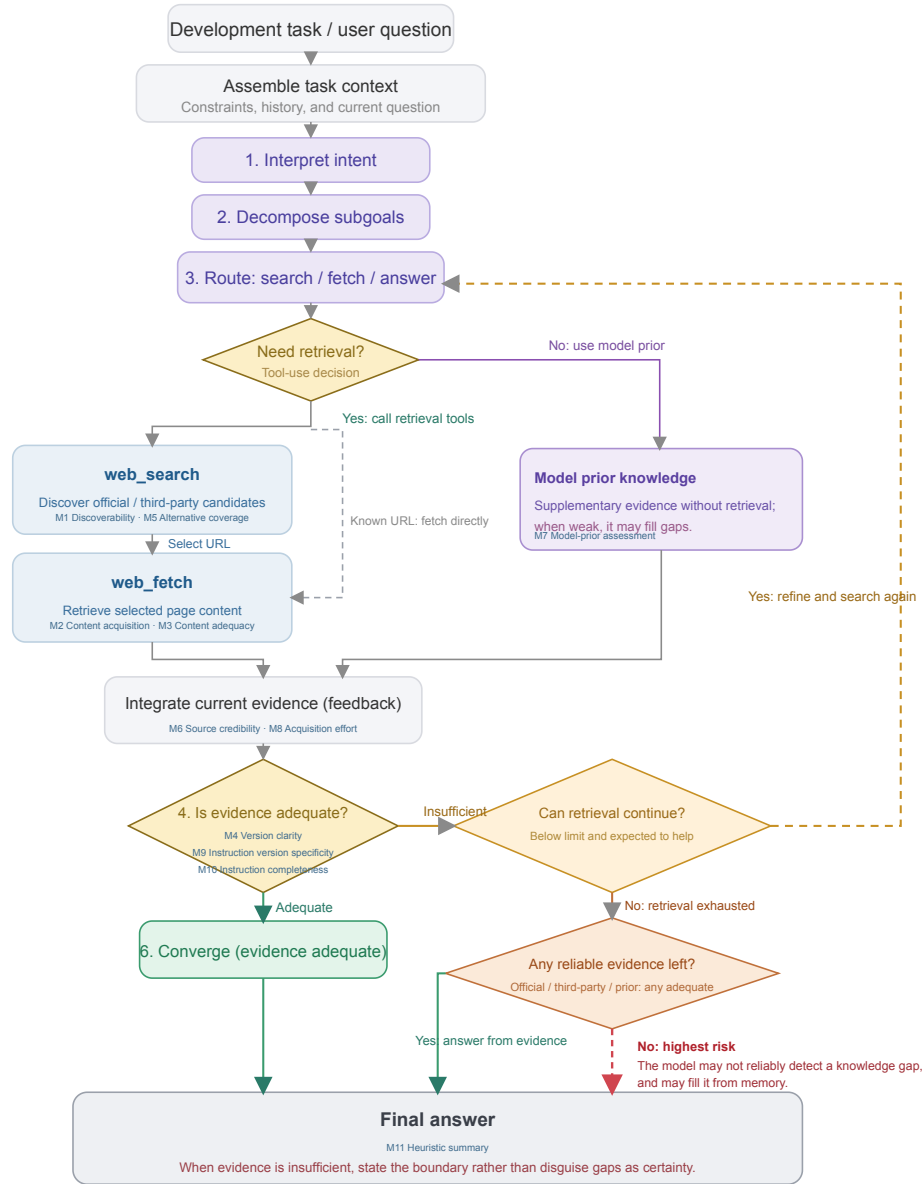
Fig. 1. An agent starts from a task and context, interprets intent, decomposes subgoals, and routes to retrieval or model prior; a retrieval branch searches, selects URLs, fetches content or fetches a known URL directly, then integrates evidence and assesses adequacy. Insufficient evidence can trigger retry; exhausted retrieval distinguishes whether reliable evidence remains.
