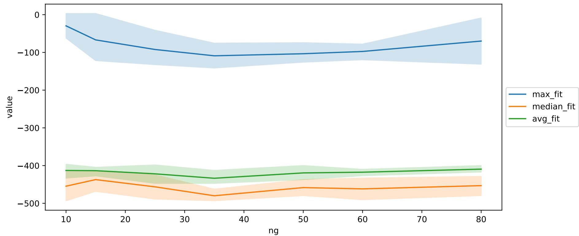
Lunar Lander-DE
