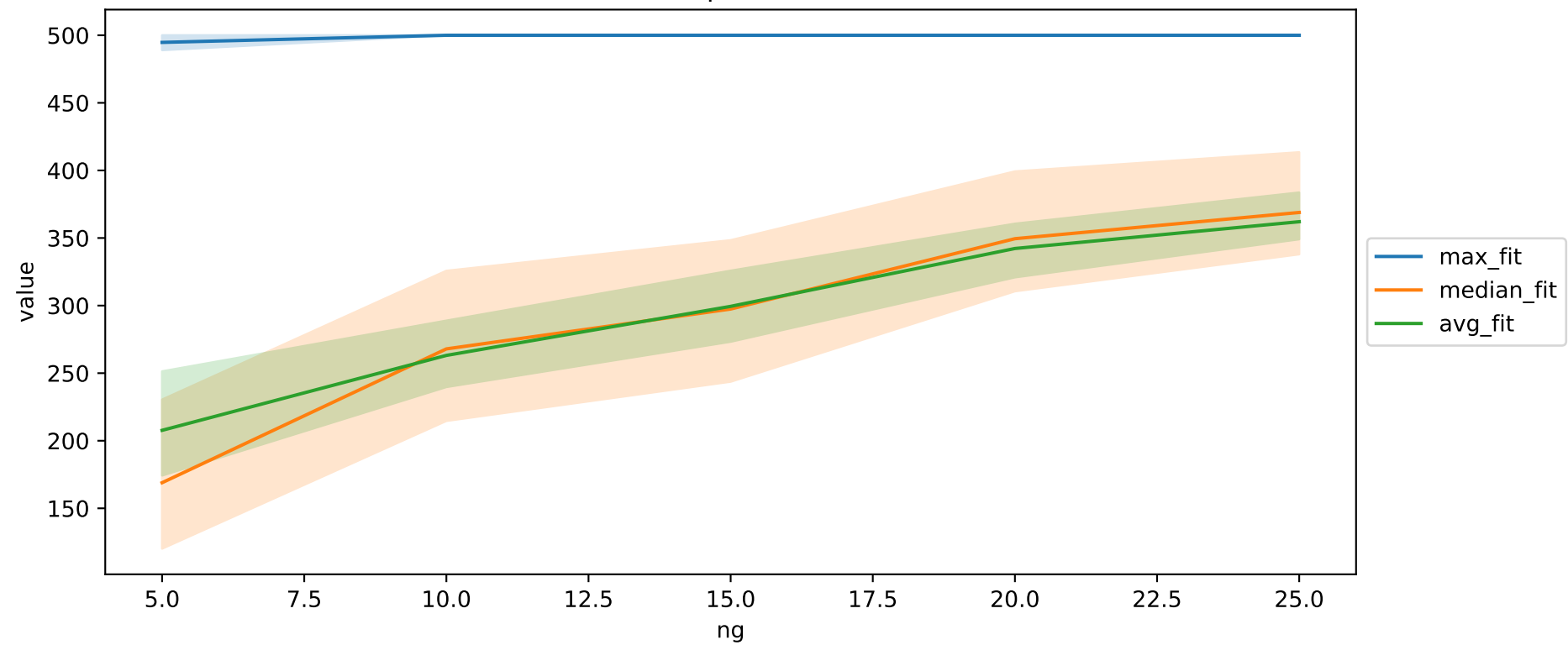
Cartpole-DE
