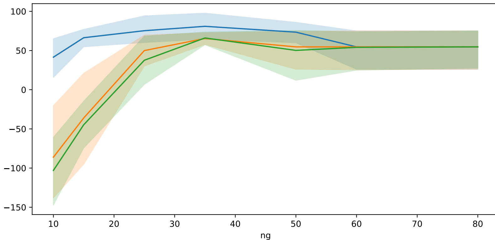
Lunar Lander-DE
