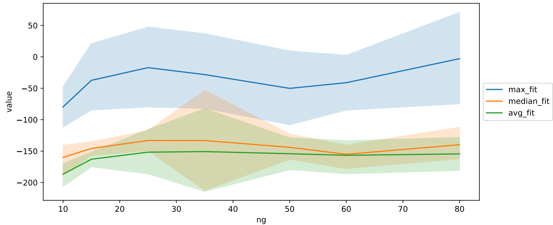
Lunar Lander-DE
