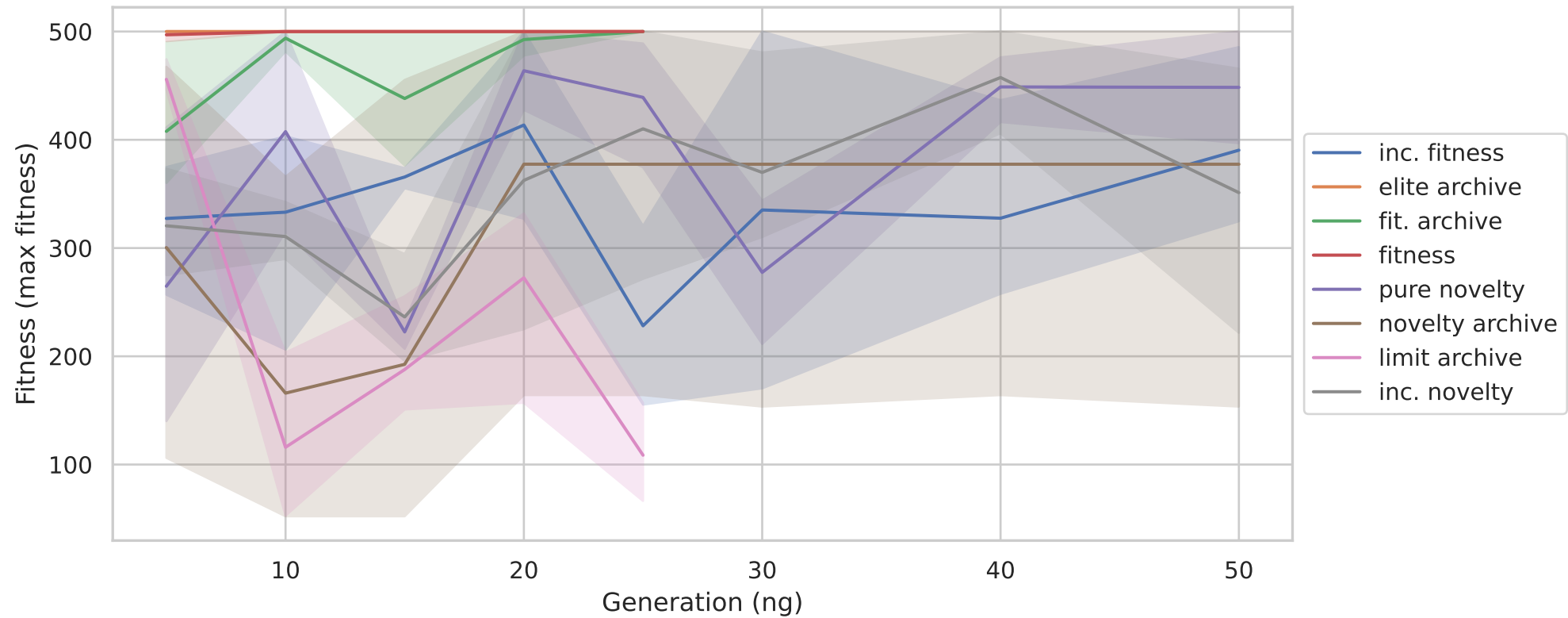
CartPole-DE
