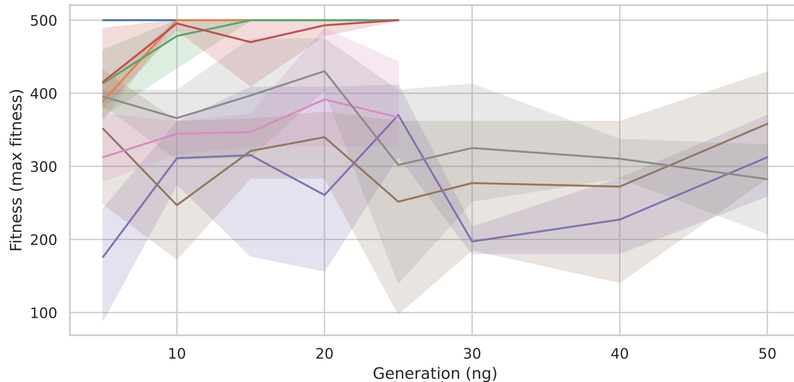
CartPole-DE
