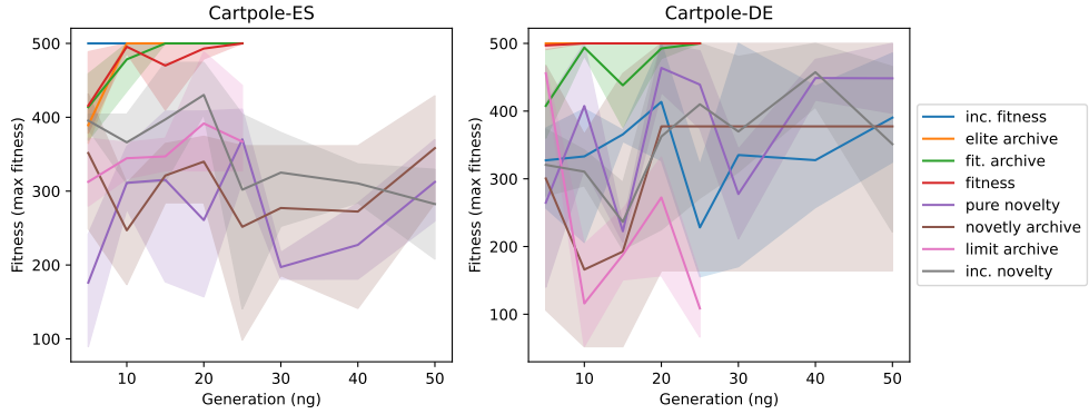
Figure 5.1: Fitness/Generation Characteristics for Cartpole environment
