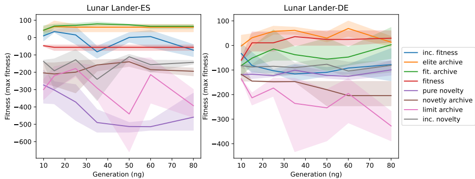
Figure 5.2: Fitness/Generation Characteristics for Lunar Lander environment (ES left, DE right)
