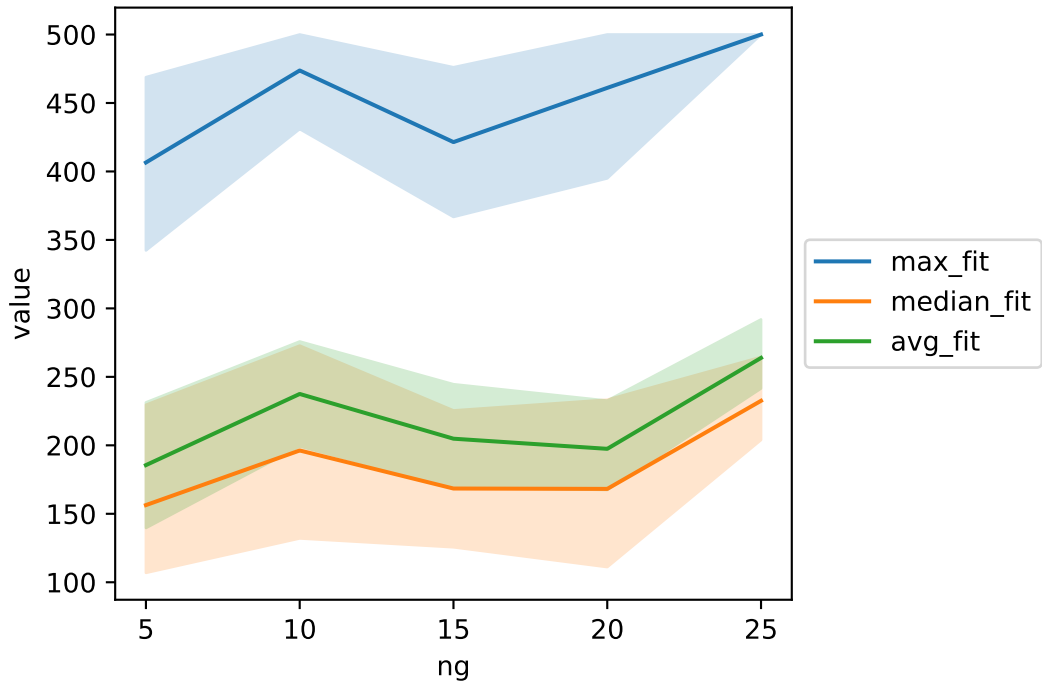
Cartpole-DE
