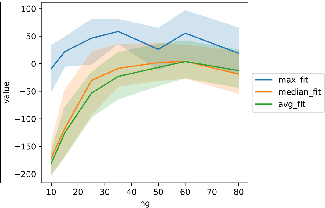
Lunar Lander-DE
