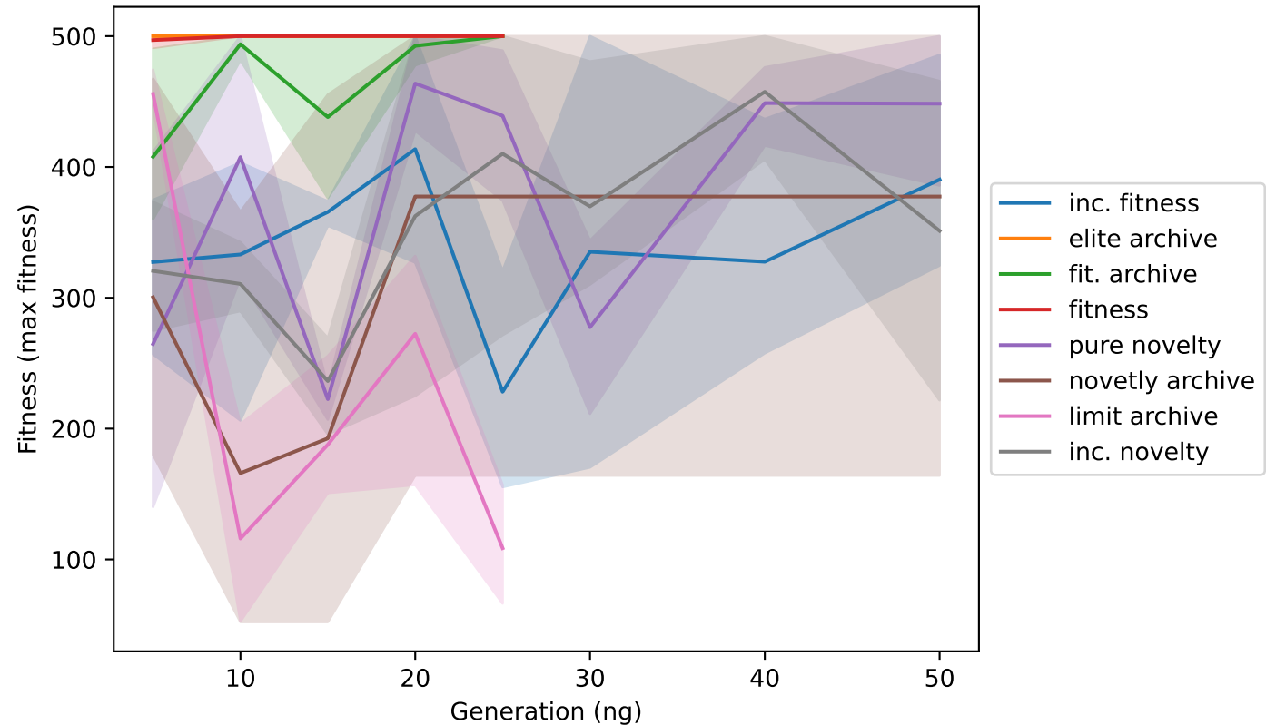
Cartpole-DE
