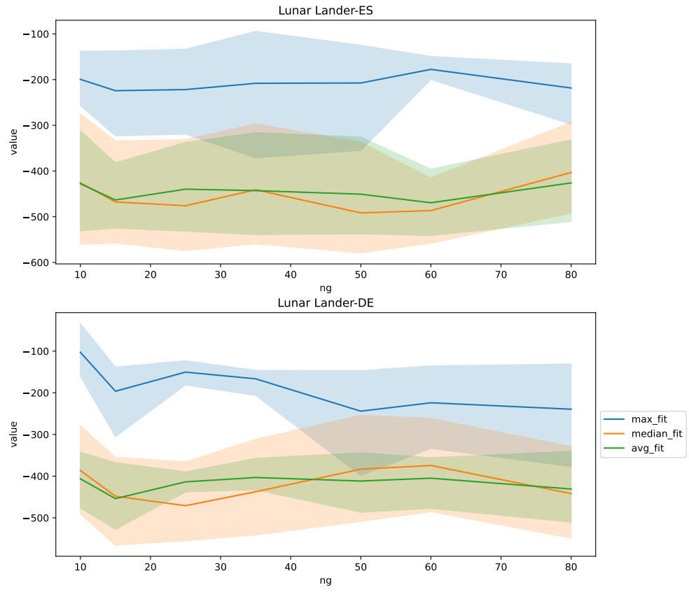
Figure A.15: Detailed fitness/generation characteristic for novelty archive on Lunar Lander env.
