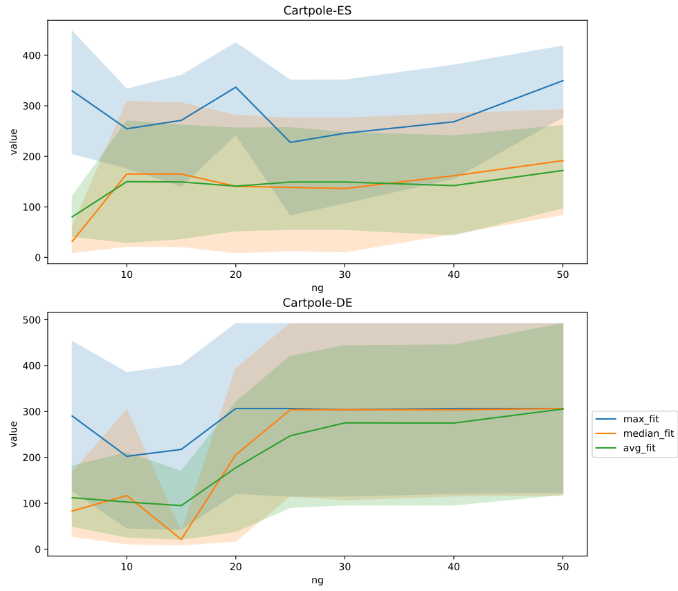
Figure A.7: Detailed fitness/generation characteristic for novelty archive on Cartpole env.
