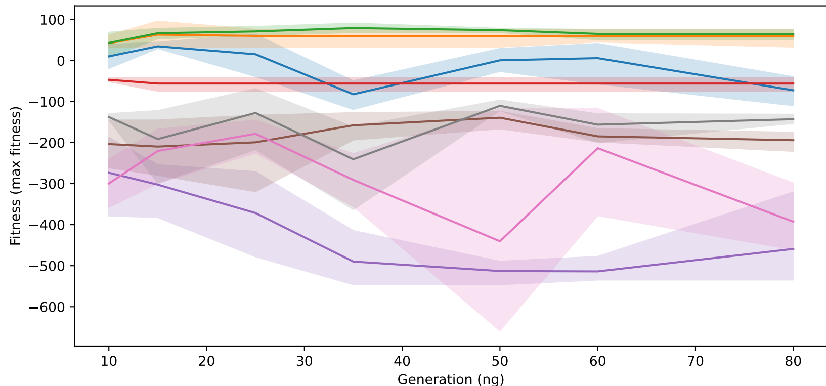
Lunar Lander-DE
