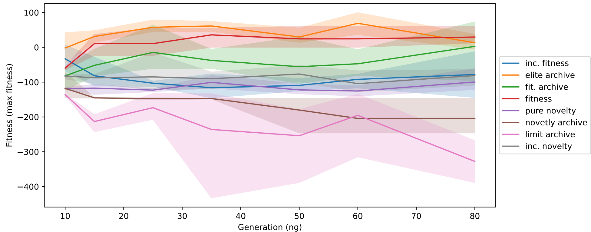
Lunar Lander-DE
