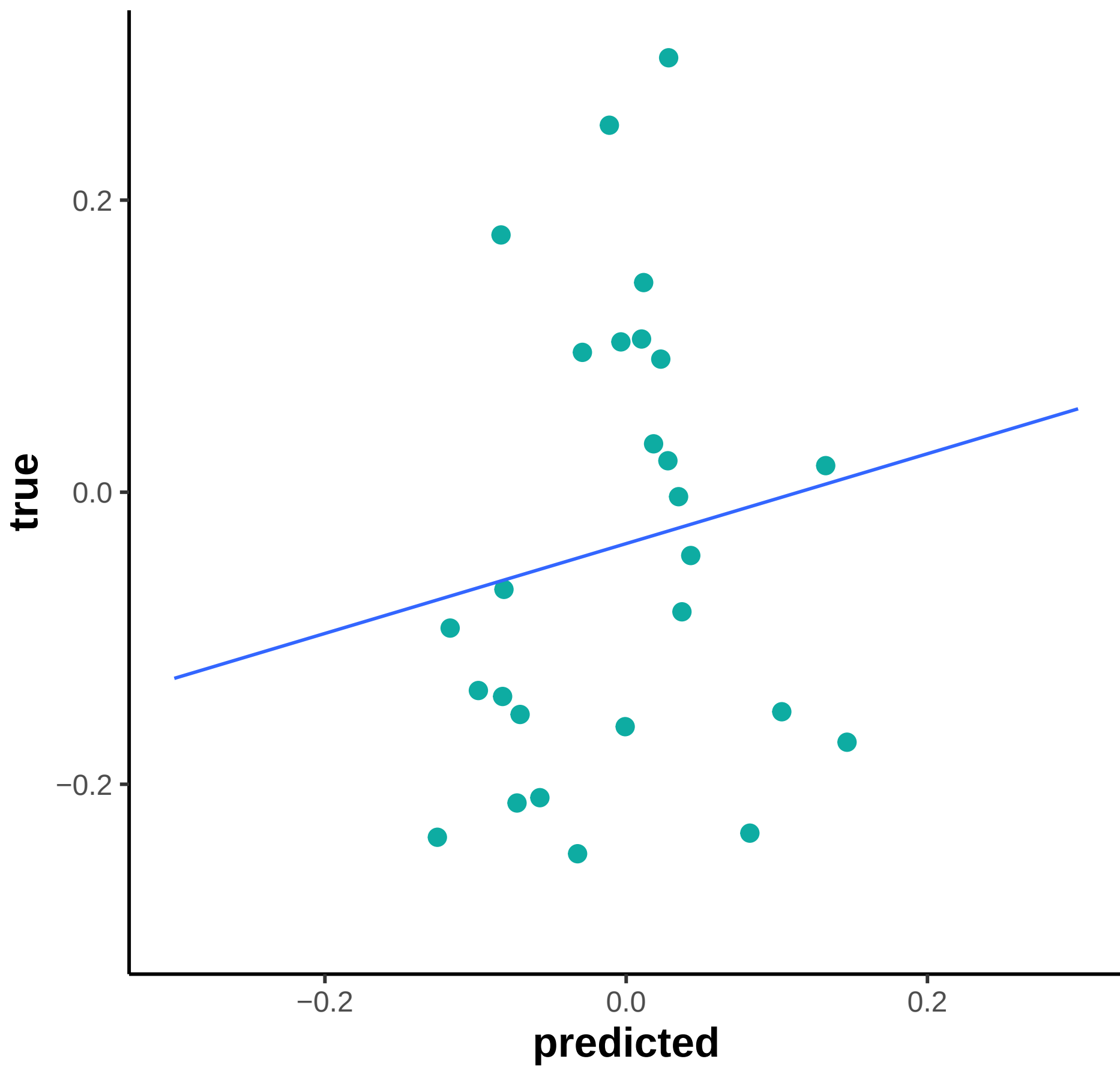
component 3
