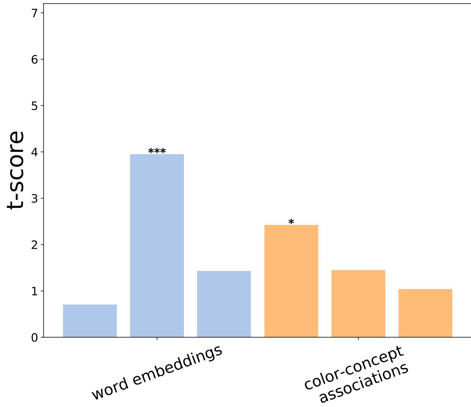
Regressor t-scores for 2nd color judgement component
