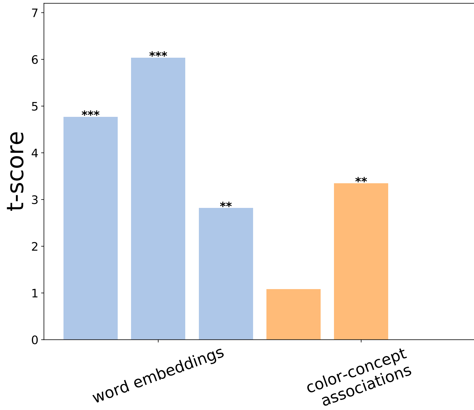
Regressor t-scores for 2nd semantic judgement component
