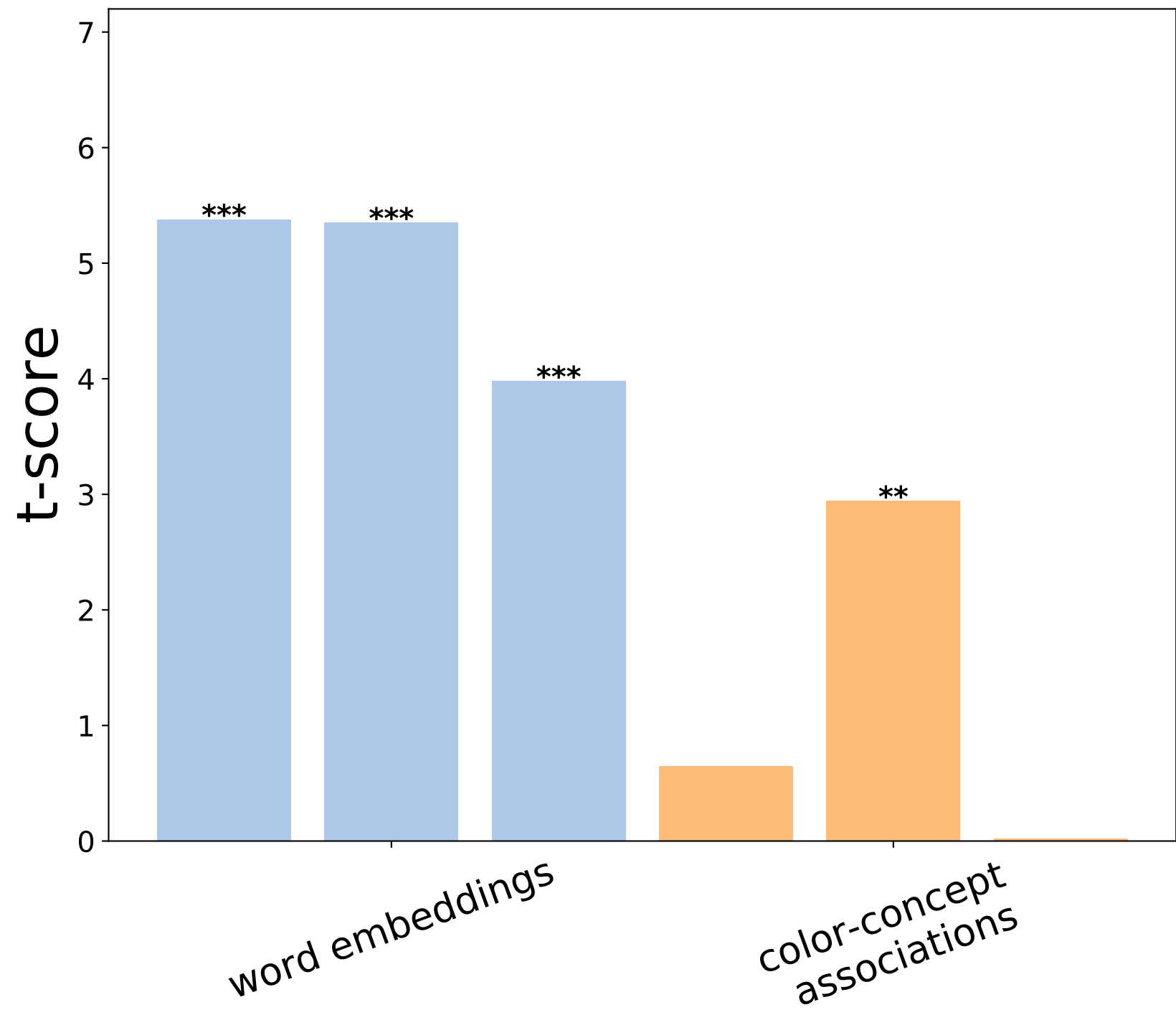
Regressor t-scores for 1st symbolic judgement component
