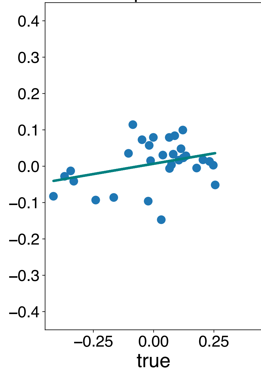
component 3
