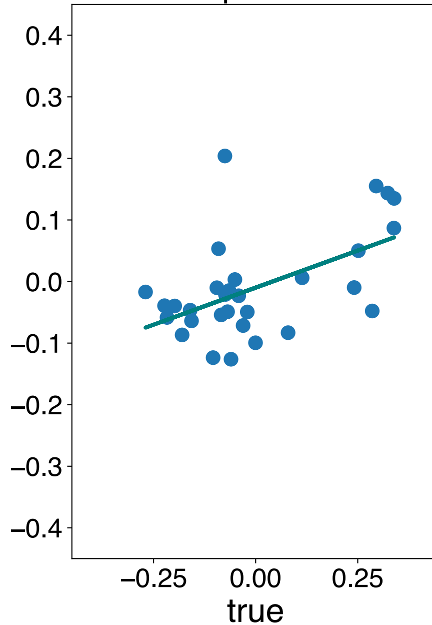
component 2
