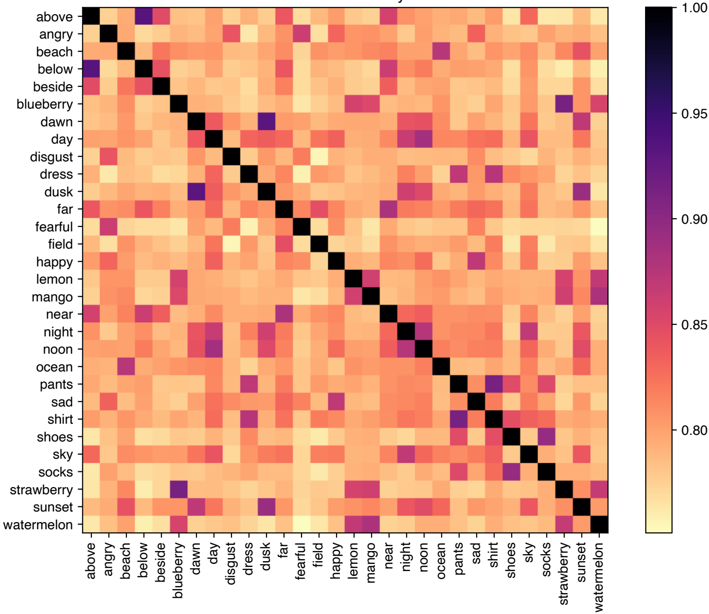
GPT-3 embed similarity matrix
