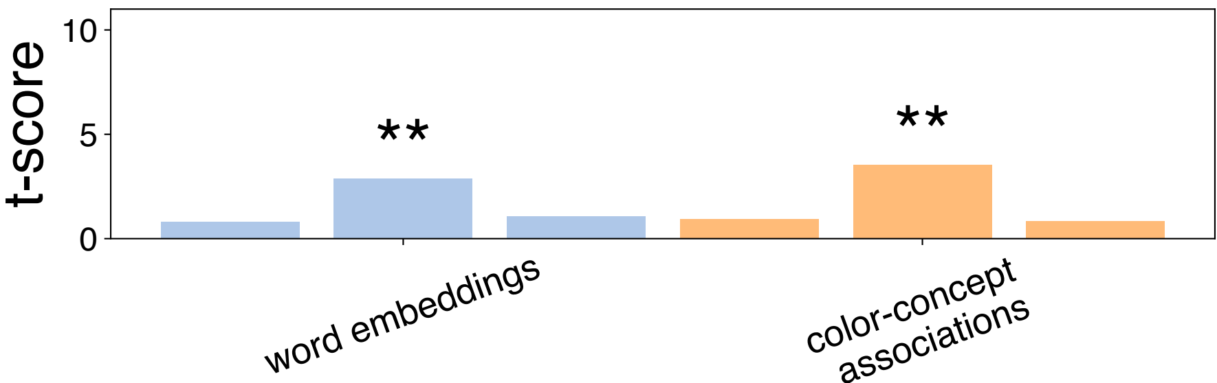
Regressor t-scores for color judgement component 2 using gpt word embeddings model R^2 = 0.505
