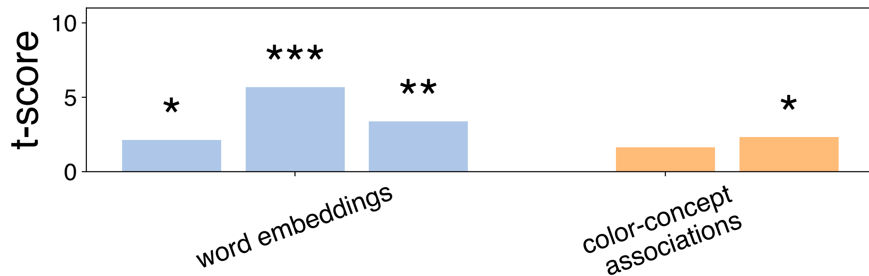
Regressor t-scores for kind judgement component 1 using fic word embeddings model R^2 = 0.774
