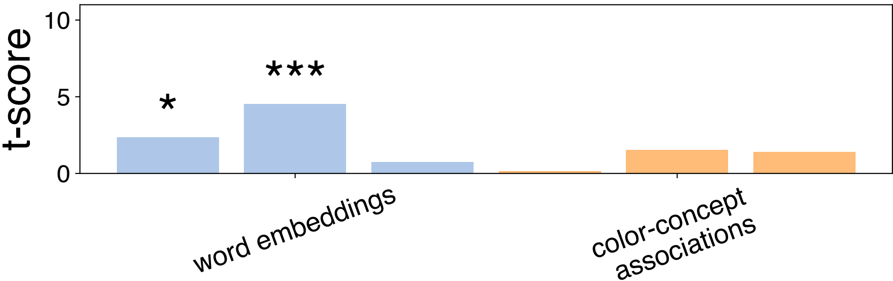
Regressor t-scores for kind judgement component 1 using gpt word embeddings model R^2 = 0.678
