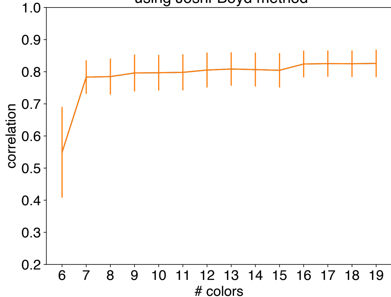
Reconstructions with 6 pcs and varying number of colors using Joshi-Boyd method
