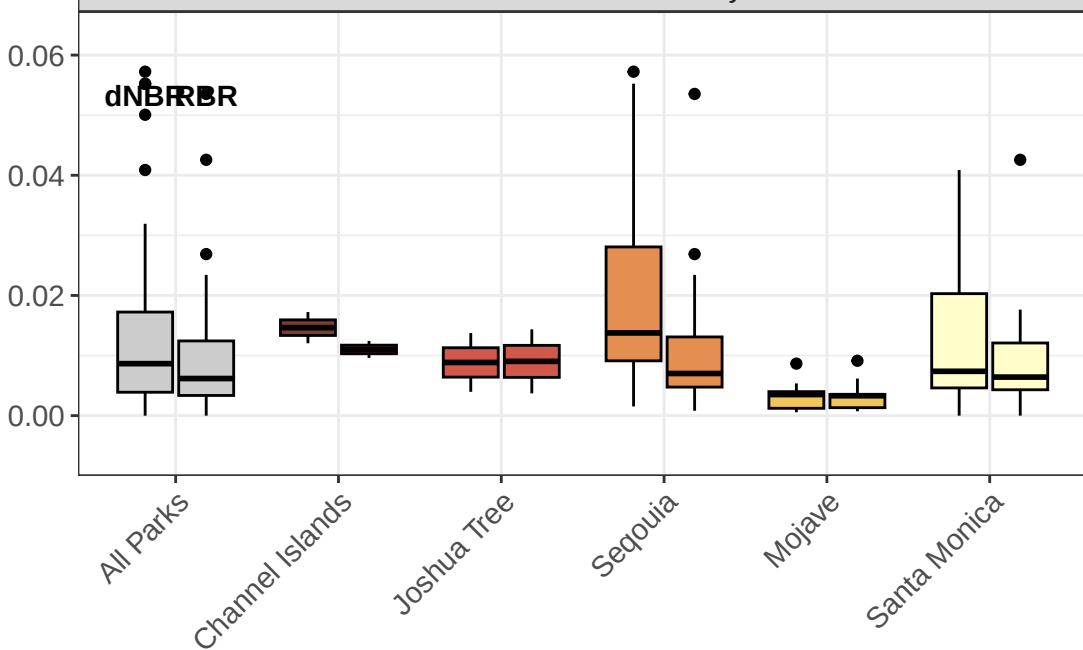
Variance of burn severity
