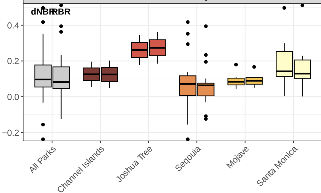
Mean burn severity
