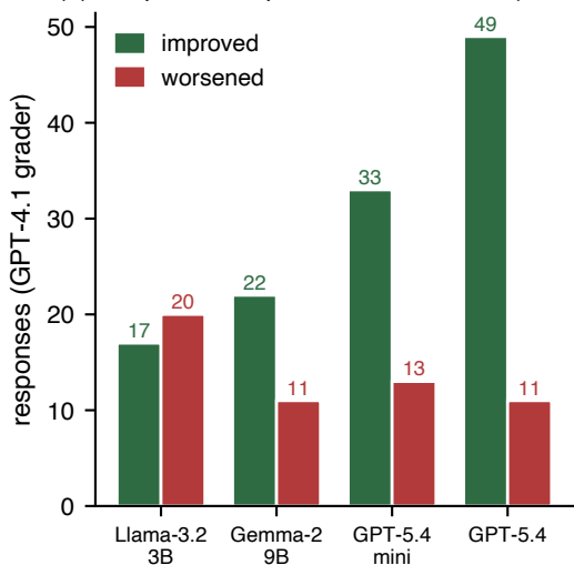
(b) Responses improved vs worsened (>0.5 pt)
