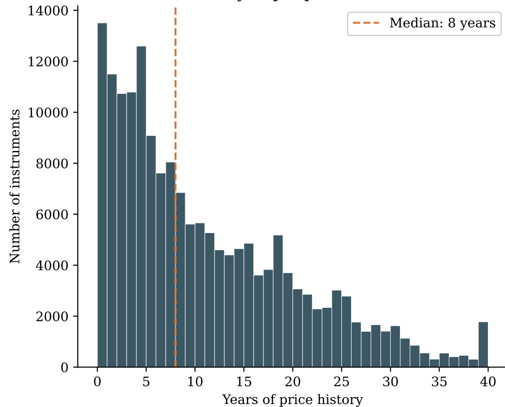
(a) History Depth per Instrument
