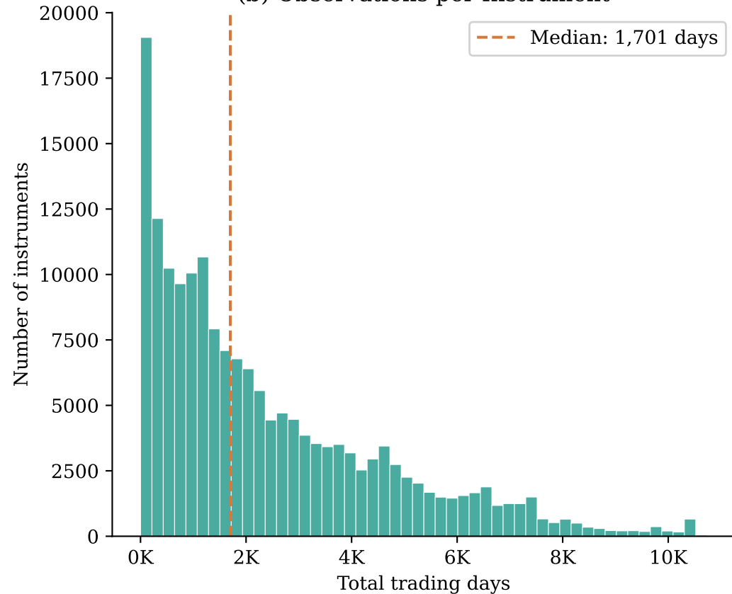
(b) Observations per Instrument
