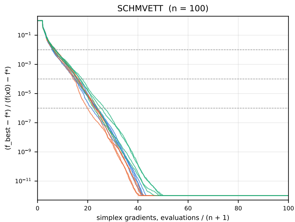
README benchmark, per-problem convergence (4 random frames, budget 100 ( n + 1 ); f^* = best value reached by any run)
