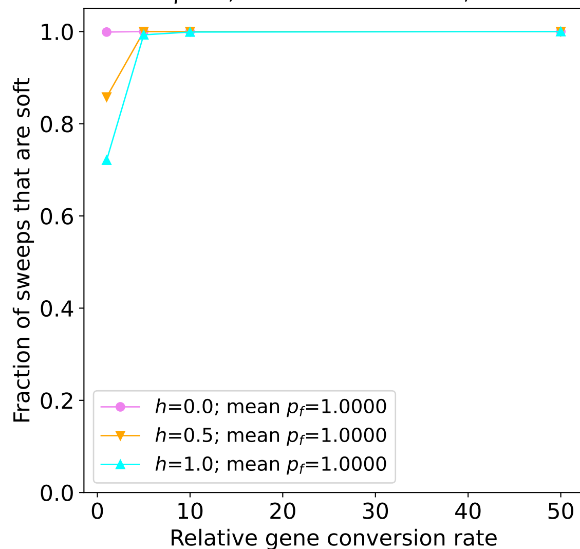
human; constant-size model; s=0.01
