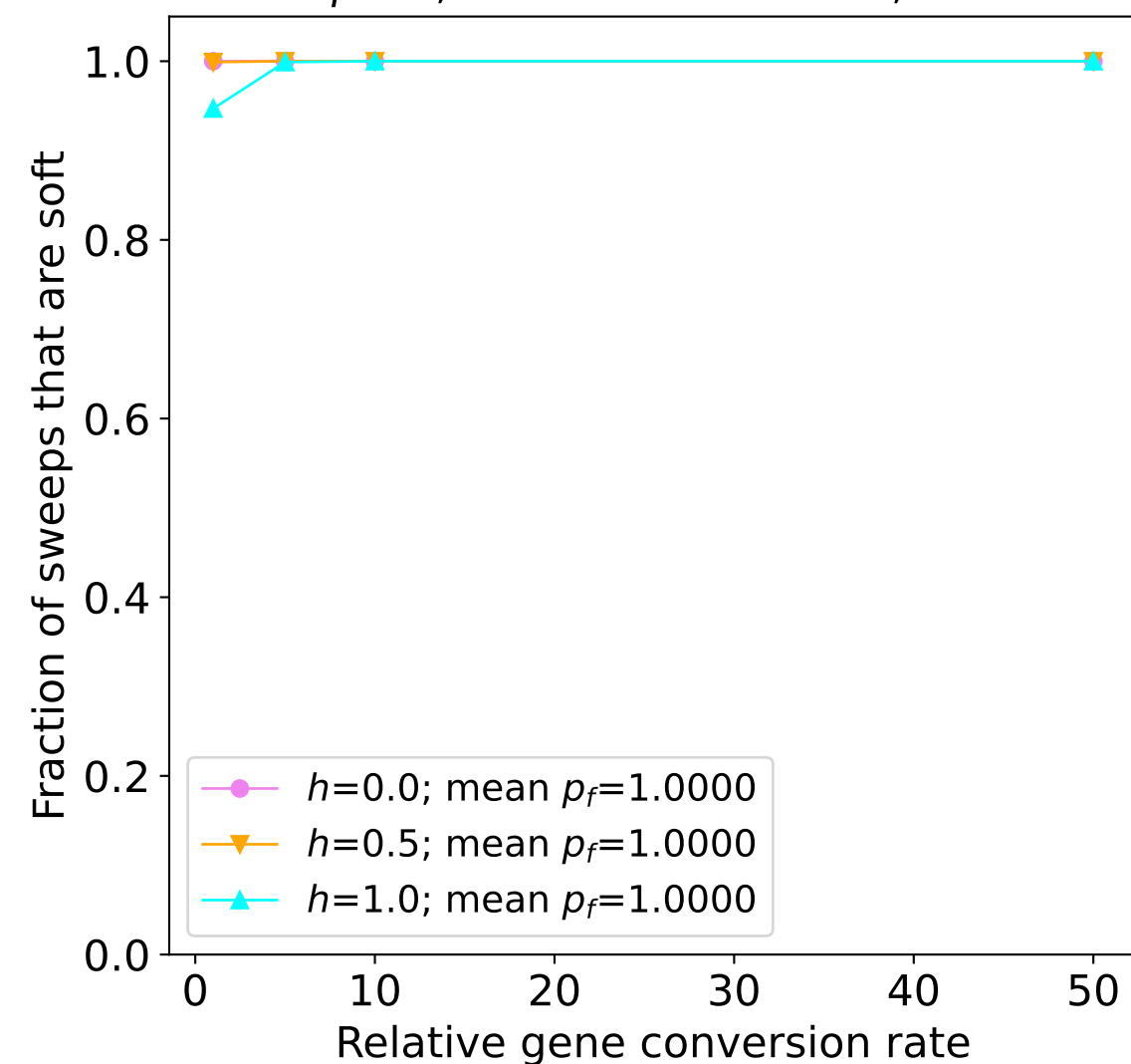
human; constant-size model; s=0.001
