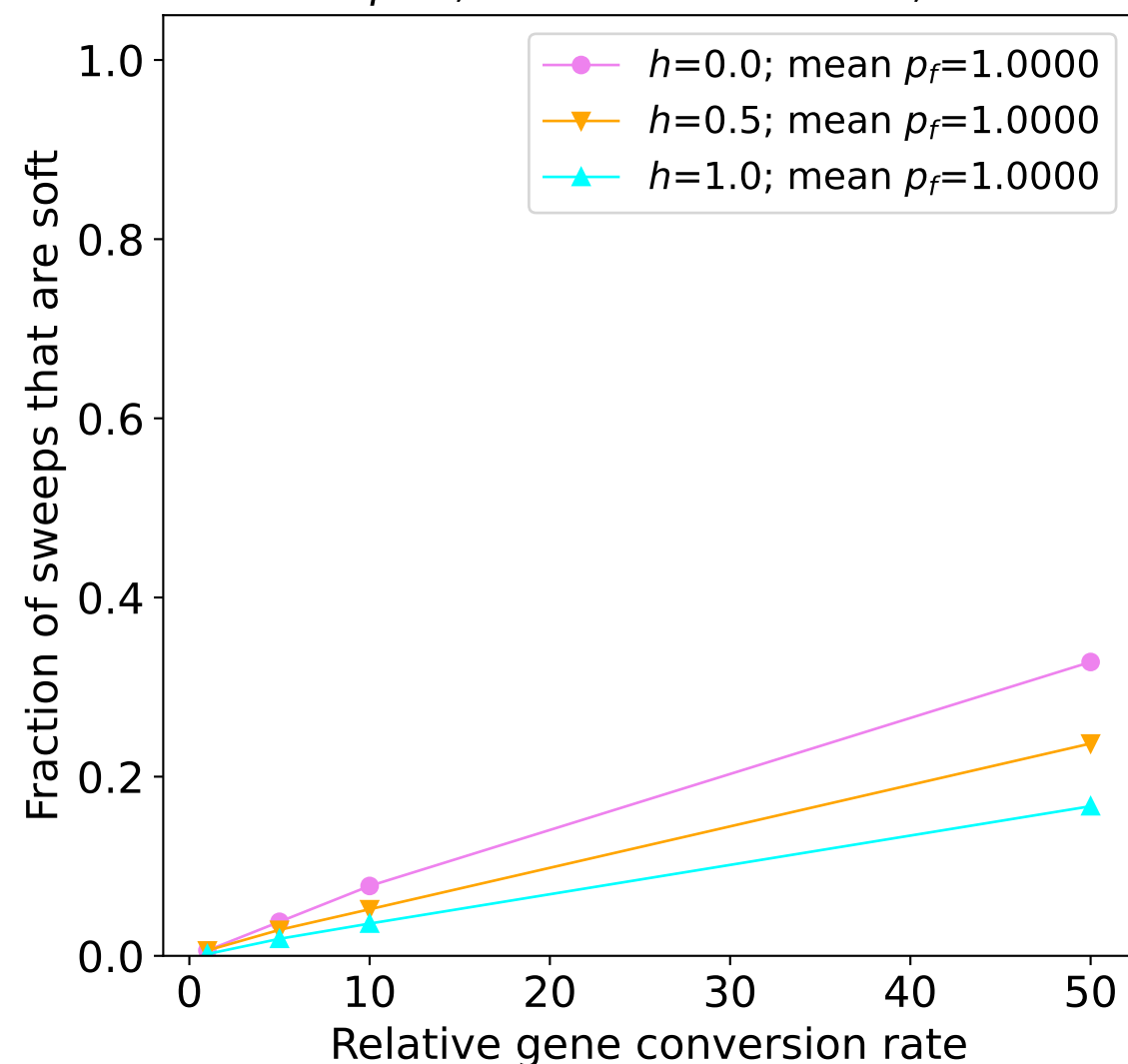
Drosophila ; constant-size model; s=0.01
