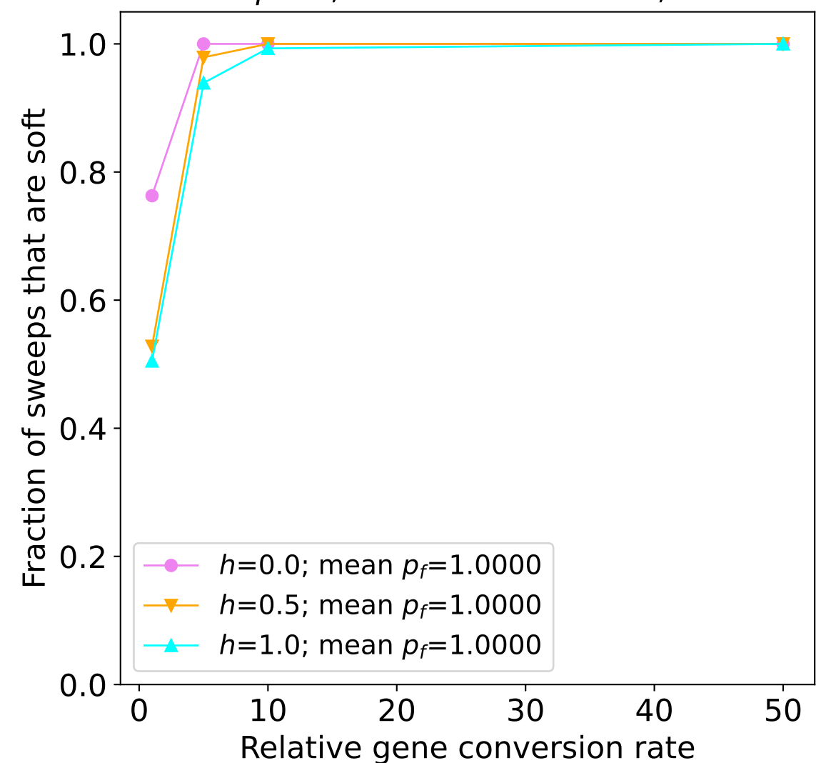
human; constant-size model; s=0.1
