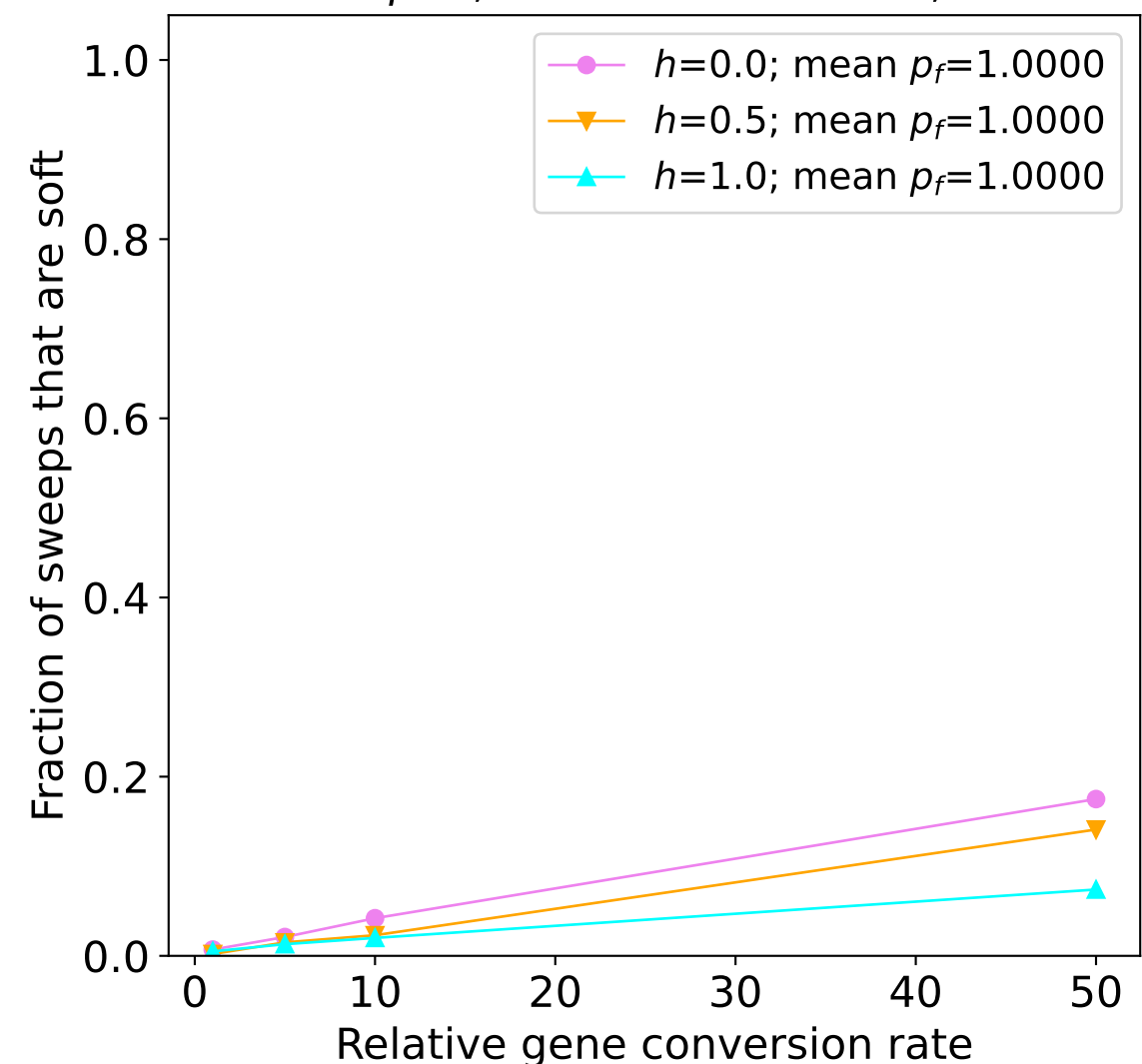
Drosophila ; constant-size model; s=0.1
