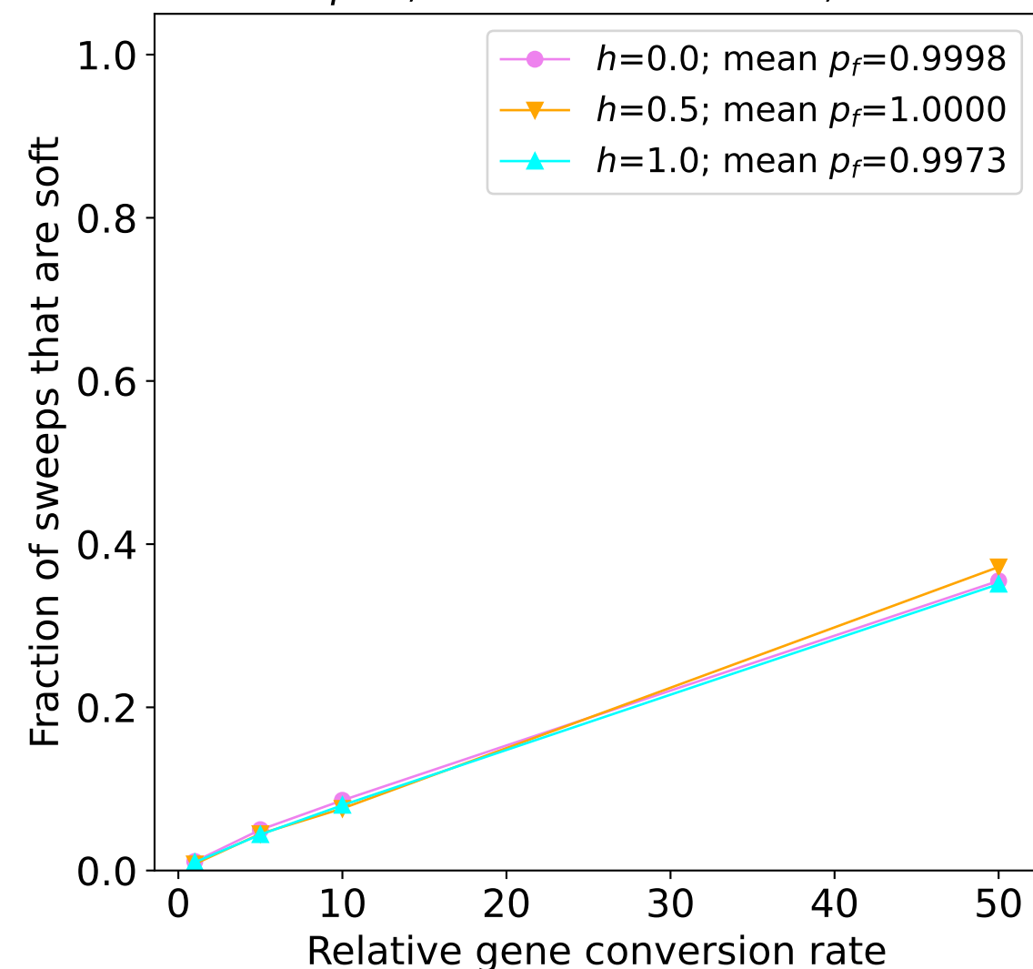
Drosophila ; constant-size model; s=0.001
