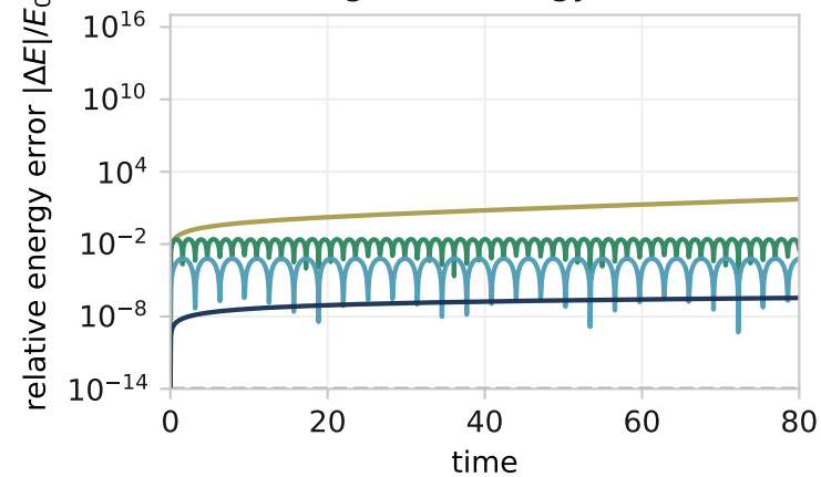
Long-time energy error
