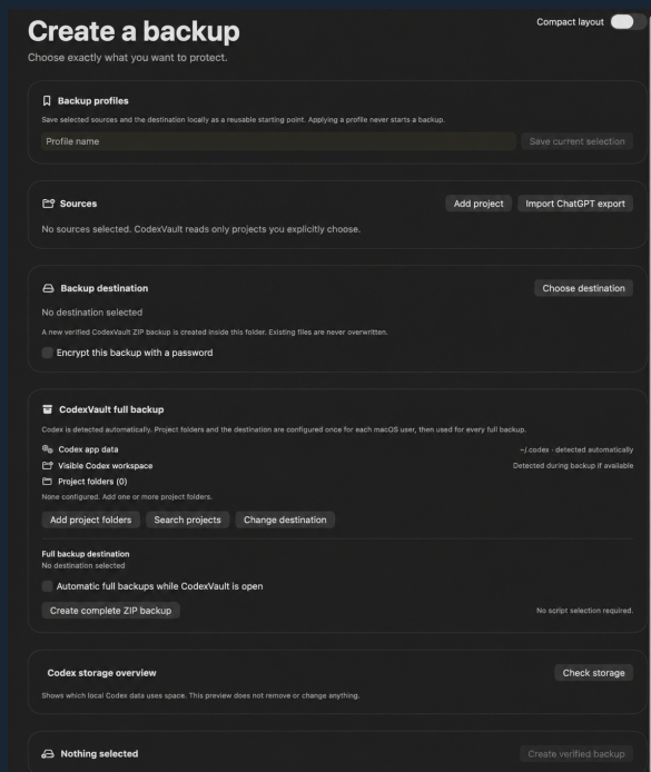
Expanded Backup view with full-backup controls and local storage overview
