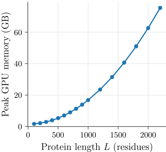
(a) Peak GPU memory
