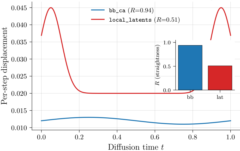
Flow-Field Curvature per Channel ( L=400 , n_{\text{samples}}=8 )
