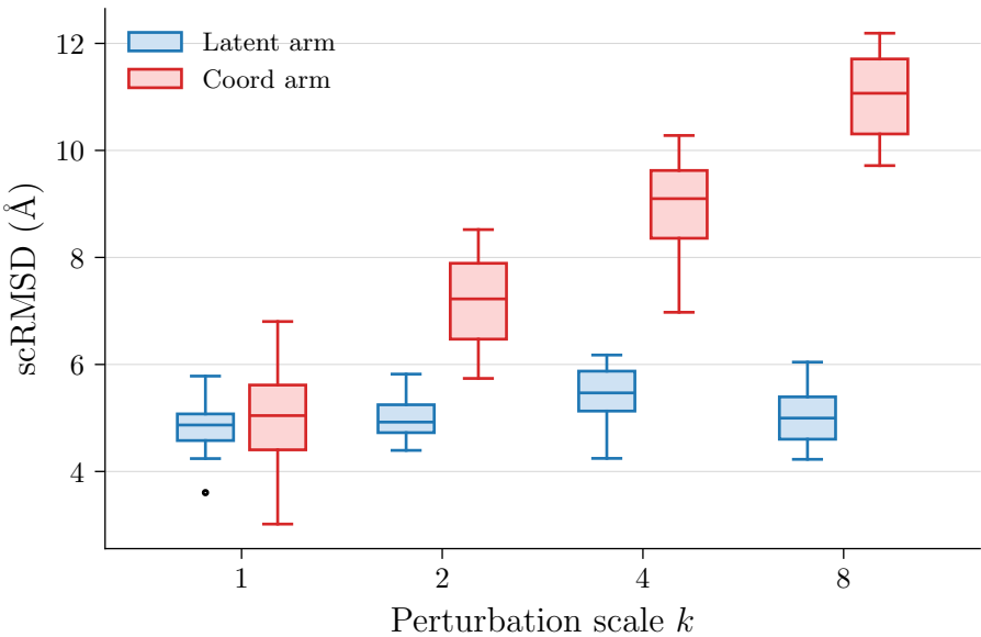
Sidechain Perturbation: Latent (contractive) vs Coord
