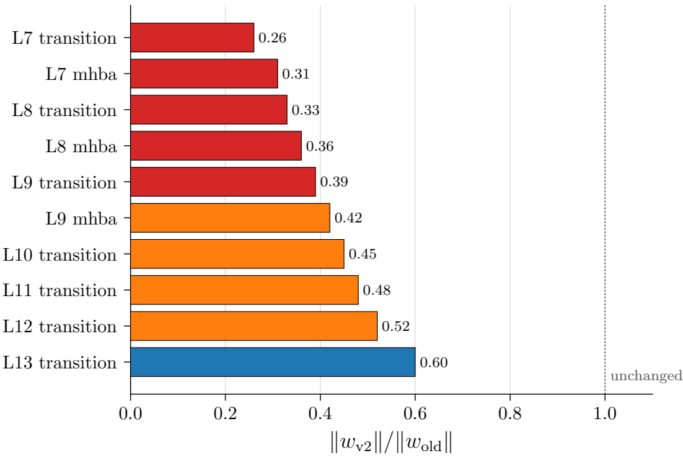
AdaLN-Zero Gate Norm Ratio (v2 / canonical), 10 Worst Layers
