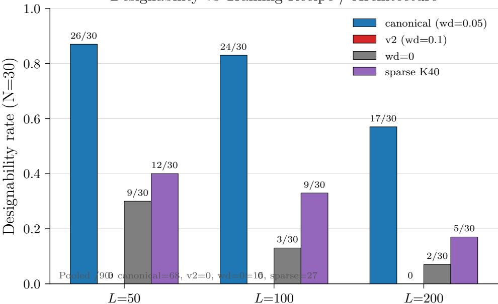
Designability vs Training Recipe / Architecture
