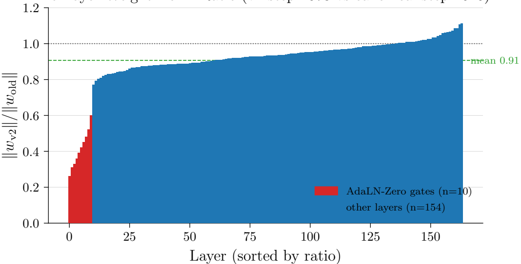
Per-layer Weight-Norm Ratio (v2 step 2078 vs canonical step 2646)
