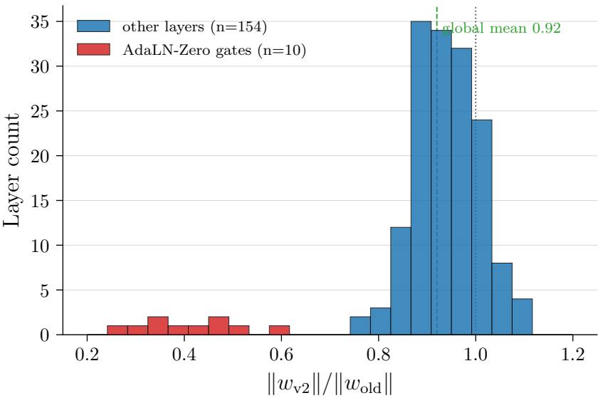
Weight-Norm Ratio Distribution: Gates Collapse, Bulk Intact
