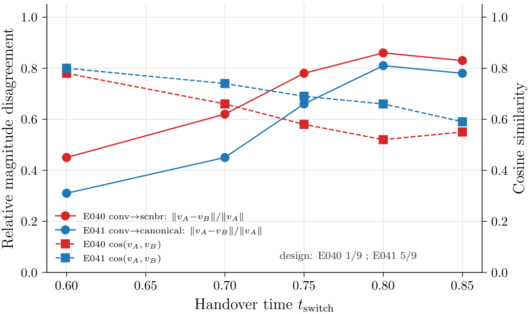
Hybrid Handover Kink: Magnitude \uparrow + Cosine \downarrow near t = 0.8
