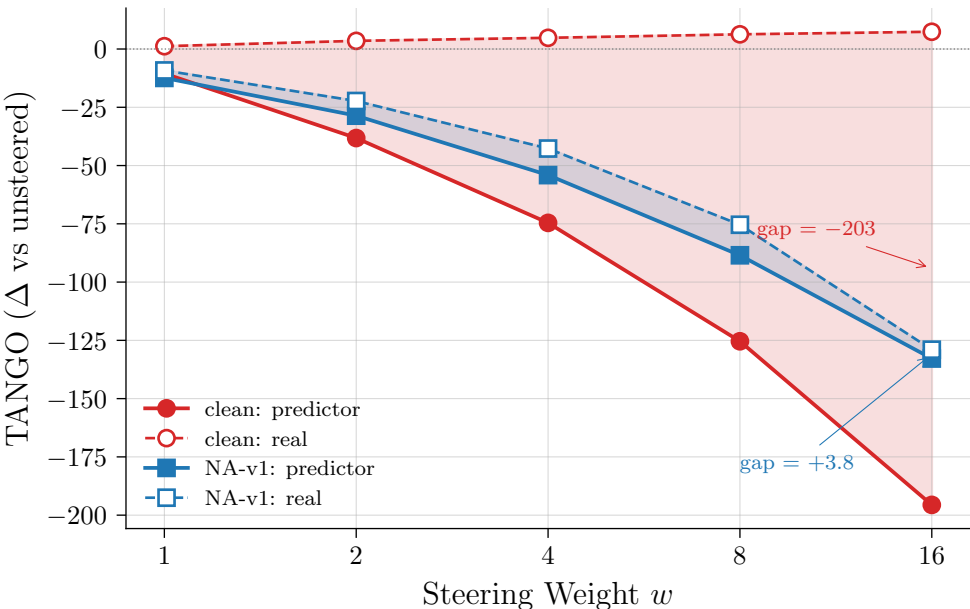
Predictor:Real Gap Closes with Noise-Aware Ensemble
