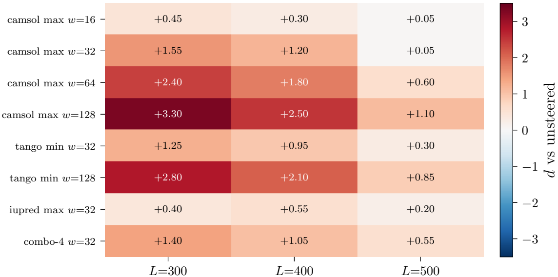
Per-Length Steering Response (Cohen's d )
