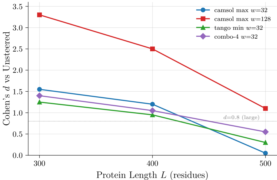
Steering Effect Decays with Length
