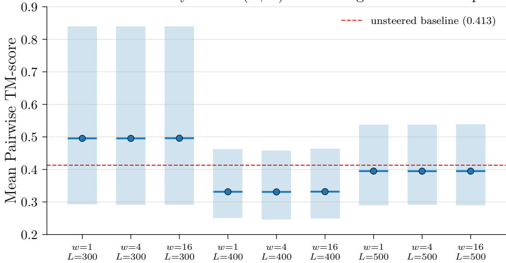
Ensemble Diversity Across (w, L) — Steering Does Not Collapse
